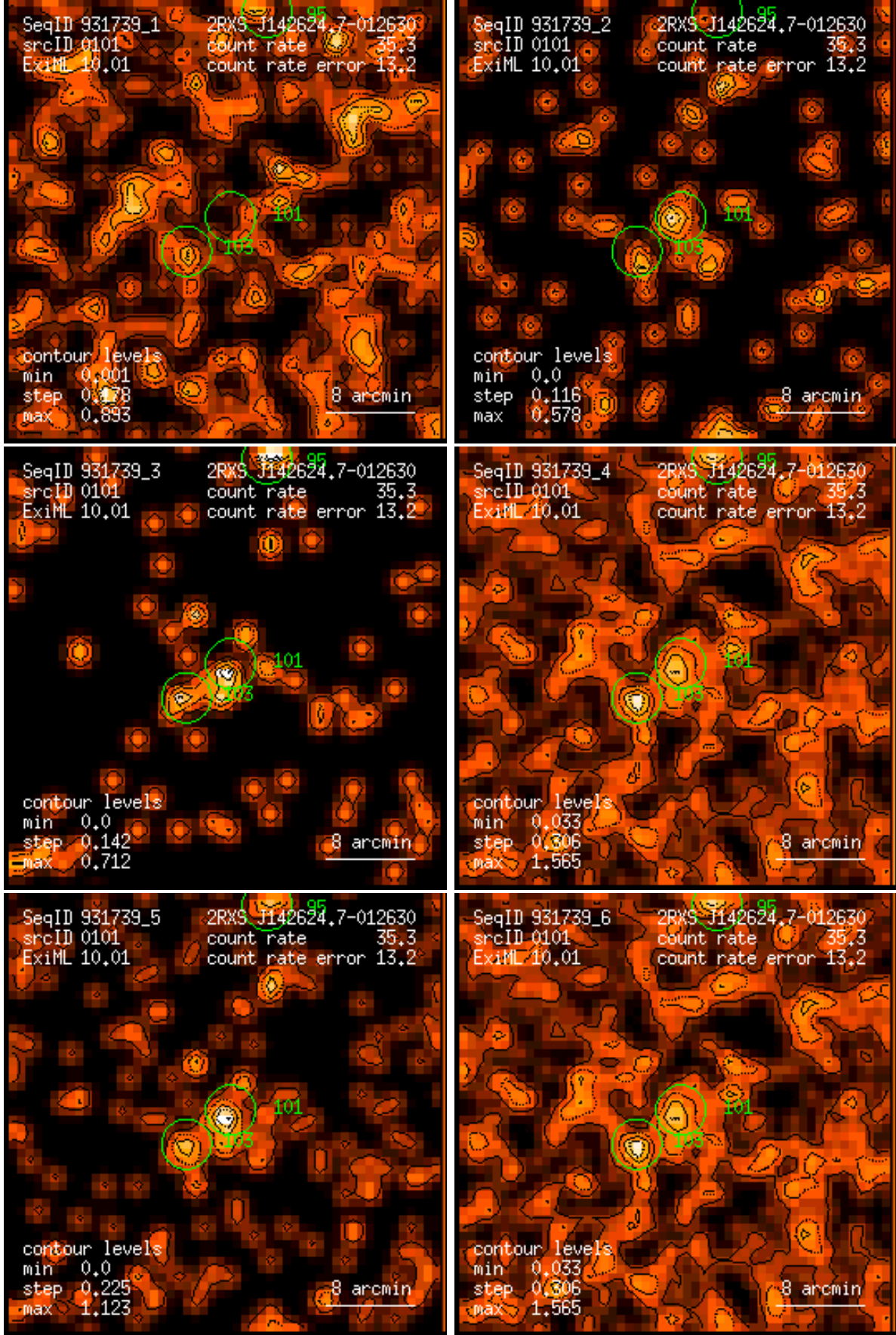
Figure 101: RASS 931739: detection 0101: band rate images, Gaussian filter: (1) PSPC channels 11 – 41, (2) 52 – 90, (3) 91 – 201, (4) 11 – 235, (5) 52 – 201, (6) 11 – 201. Broad band rates in counts/ks. Band rate contour levels in counts/ks/arcmin 2 .
