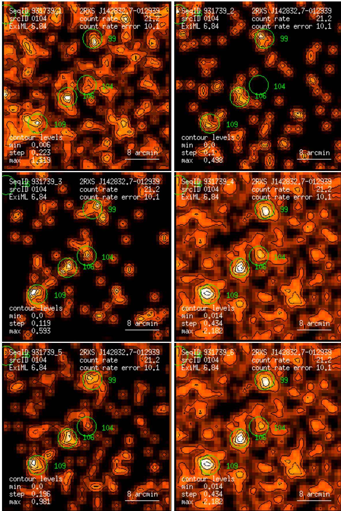
Figure 104: RASS 931739: detection 0104: band rate images, Gaussian filter: (1) PSPC channels 11 – 41, (2) 52 – 90, (3) 91 – 201, (4) 11 – 235, (5) 52 – 201, (6) 11 – 201. Broad band rates in counts/ks. Band rate contour levels in counts/ks/arcmin 2 .
