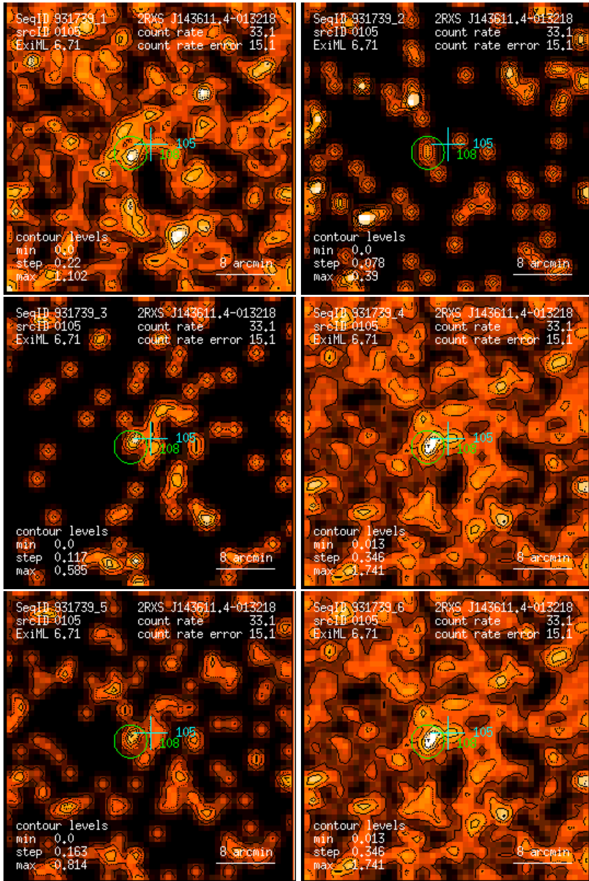
Figure 105: RASS 931739: detection 0105: band rate images, Gaussian filter: (1) PSPC channels 11 – 41, (2) 52 – 90, (3) 91 – 201, (4) 11 – 235, (5) 52 – 201, (6) 11 – 201. Broad band rates in counts/ks. Band rate contour levels in counts/ks/arcmin 2 .
