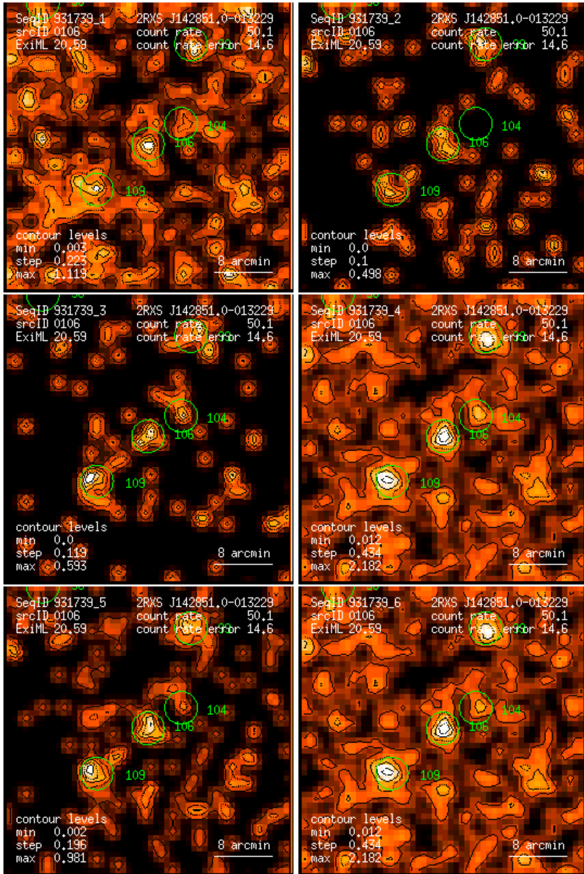
Figure 106: RASS 931739: detection 0106: band rate images, Gaussian filter: (1) PSPC channels 11 – 41, (2) 52 – 90, (3) 91 – 201, (4) 11 – 235, (5) 52 – 201, (6) 11 – 201. Broad band rates in counts/ks. Band rate contour levels in counts/ks/arcmin 2 .
