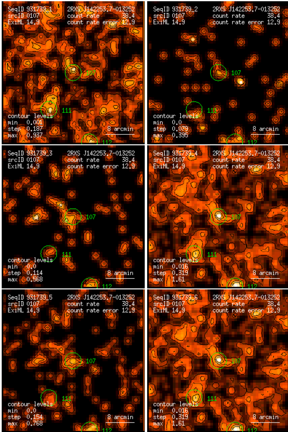
Figure 107: RASS 931739: detection 0107: band rate images, Gaussian filter: (1) PSPC channels 11 – 41, (2) 52 – 90, (3) 91 – 201, (4) 11 – 235, (5) 52 – 201, (6) 11 – 201. Broad band rates in counts/ks. Band rate contour levels in counts/ks/arcmin 2 .
