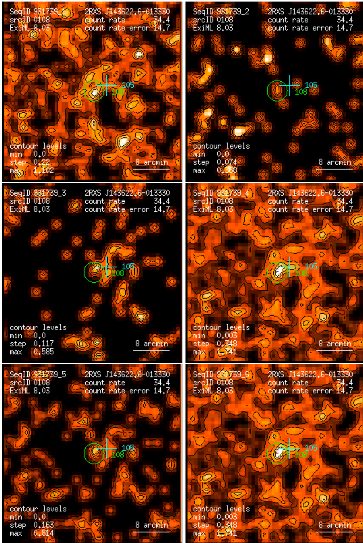
Figure 108: RASS 931739: detection 0108: band rate images, Gaussian filter: (1) PSPC channels 11 – 41, (2) 52 – 90, (3) 91 – 201, (4) 11 – 235, (5) 52 – 201, (6) 11 – 201. Broad band rates in counts/ks. Band rate contour levels in counts/ks/arcmin 2 .
