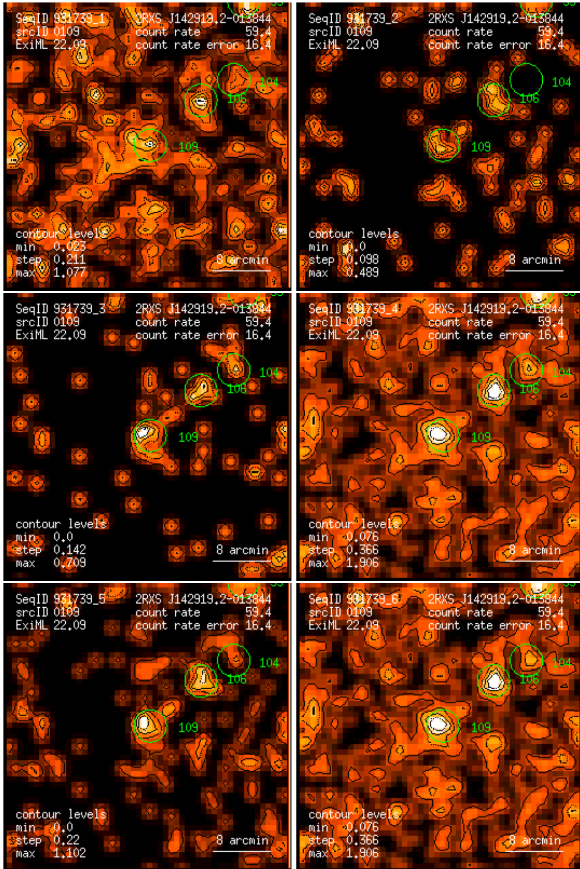
Figure 109: RASS 931739: detection 0109: band rate images, Gaussian filter: (1) PSPC channels 11 – 41, (2) 52 – 90, (3) 91 – 201, (4) 11 – 235, (5) 52 – 201, (6) 11 – 201. Broad band rates in counts/ks. Band rate contour levels in counts/ks/arcmin 2 .
