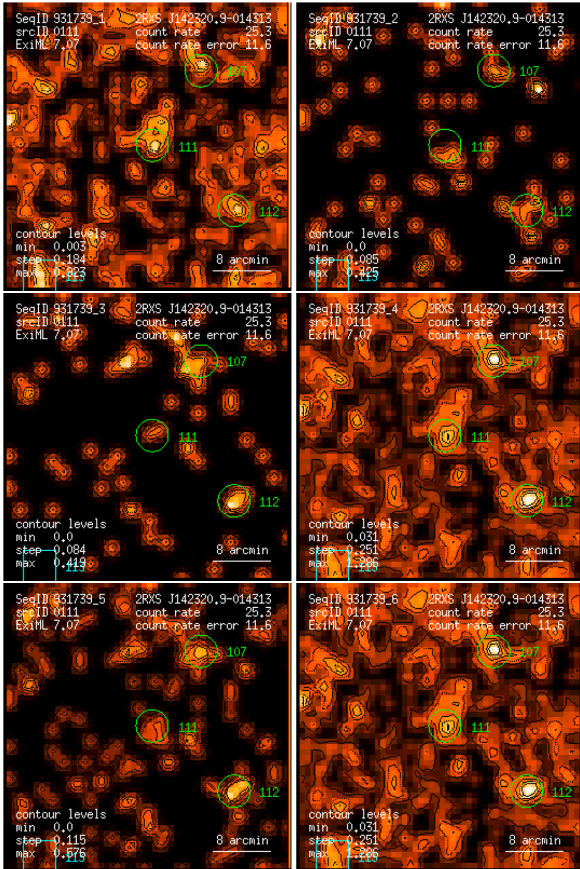
Figure 111: RASS 931739: detection 0111: band rate images, Gaussian filter: (1) PSPC channels 11 – 41, (2) 52 – 90, (3) 91 – 201, (4) 11 – 235, (5) 52 – 201, (6) 11 – 201. Broad band rates in counts/ks. Band rate contour levels in counts/ks/arcmin 2 .
