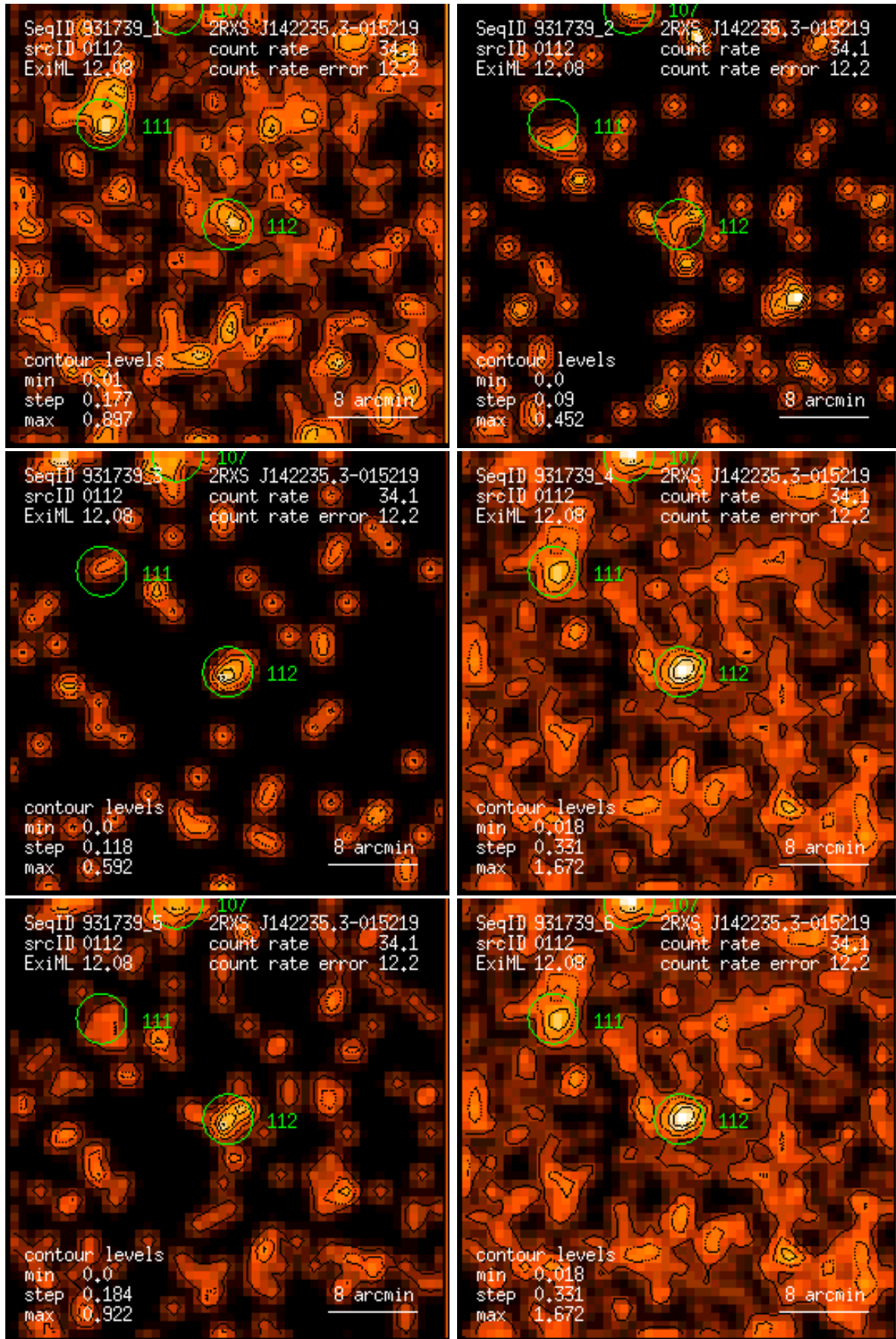
Figure 112: RASS 931739: detection 0112: band rate images, Gaussian filter: (1) PSPC channels 11 – 41, (2) 52 – 90, (3) 91 – 201, (4) 11 – 235, (5) 52 – 201, (6) 11 – 201. Broad band rates in counts/ks. Band rate contour levels in counts/ks/arcmin 2 .
