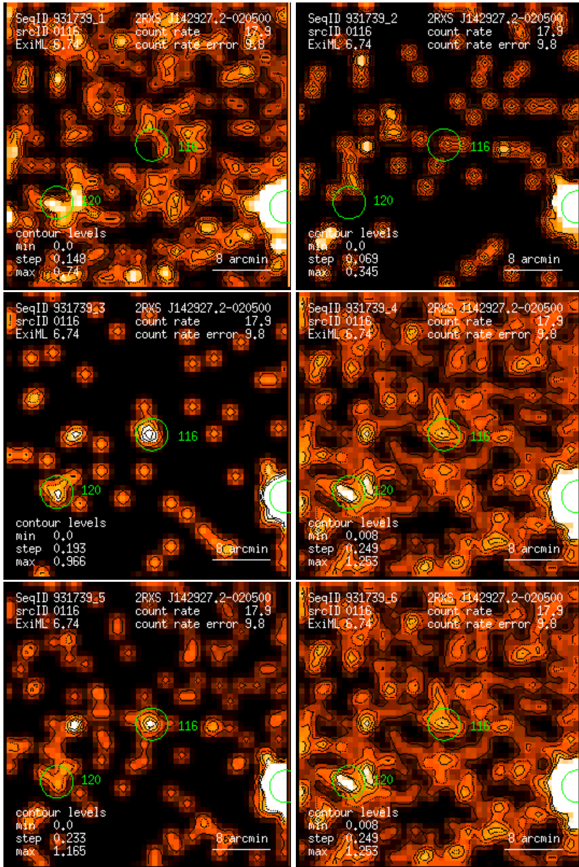
Figure 116: RASS 931739: detection 0116: band rate images, Gaussian filter: (1) PSPC channels 11 – 41, (2) 52 – 90, (3) 91 – 201, (4) 11 – 235, (5) 52 – 201, (6) 11 – 201. Broad band rates in counts/ks. Band rate contour levels in counts/ks/arcmin 2 .
