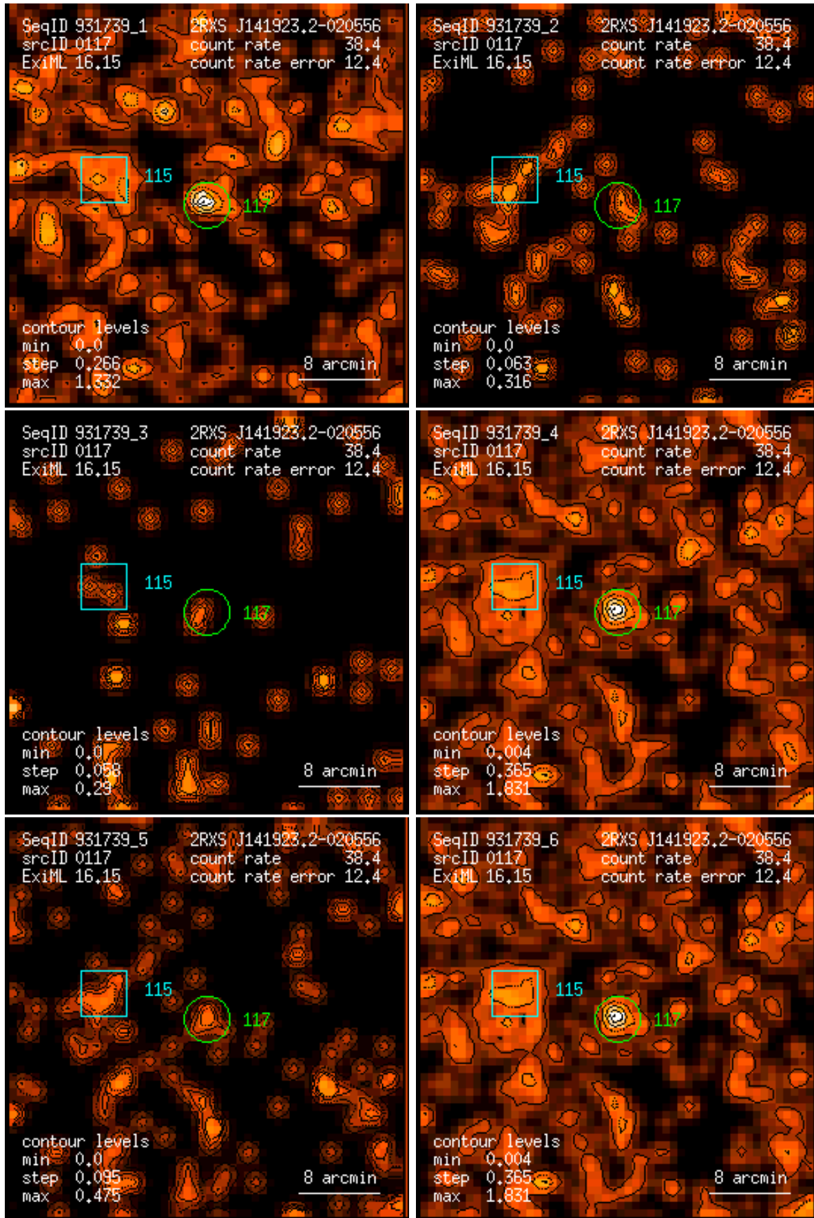
Figure 117: RASS 931739: detection 0117: band rate images, Gaussian filter: (1) PSPC channels 11 – 41, (2) 52 – 90, (3) 91 – 201, (4) 11 – 235, (5) 52 – 201, (6) 11 – 201. Broad band rates in counts/ks. Band rate contour levels in counts/ks/arcmin 2 .
