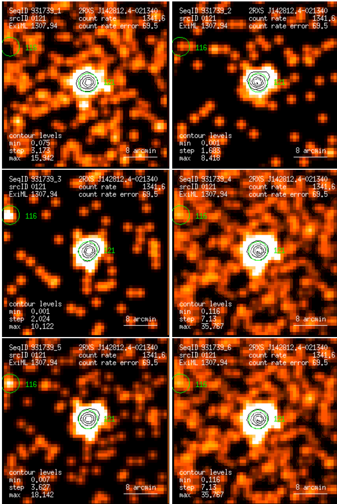
Figure 121: RASS 931739: detection 0121: band rate images, Gaussian filter: (1) PSPC channels 11 – 41, (2) 52 – 90, (3) 91 – 201, (4) 11 – 235, (5) 52 – 201, (6) 11 – 201. Broad band rates in counts/ks. Band rate contour levels in counts/ks/arcmin 2 .
