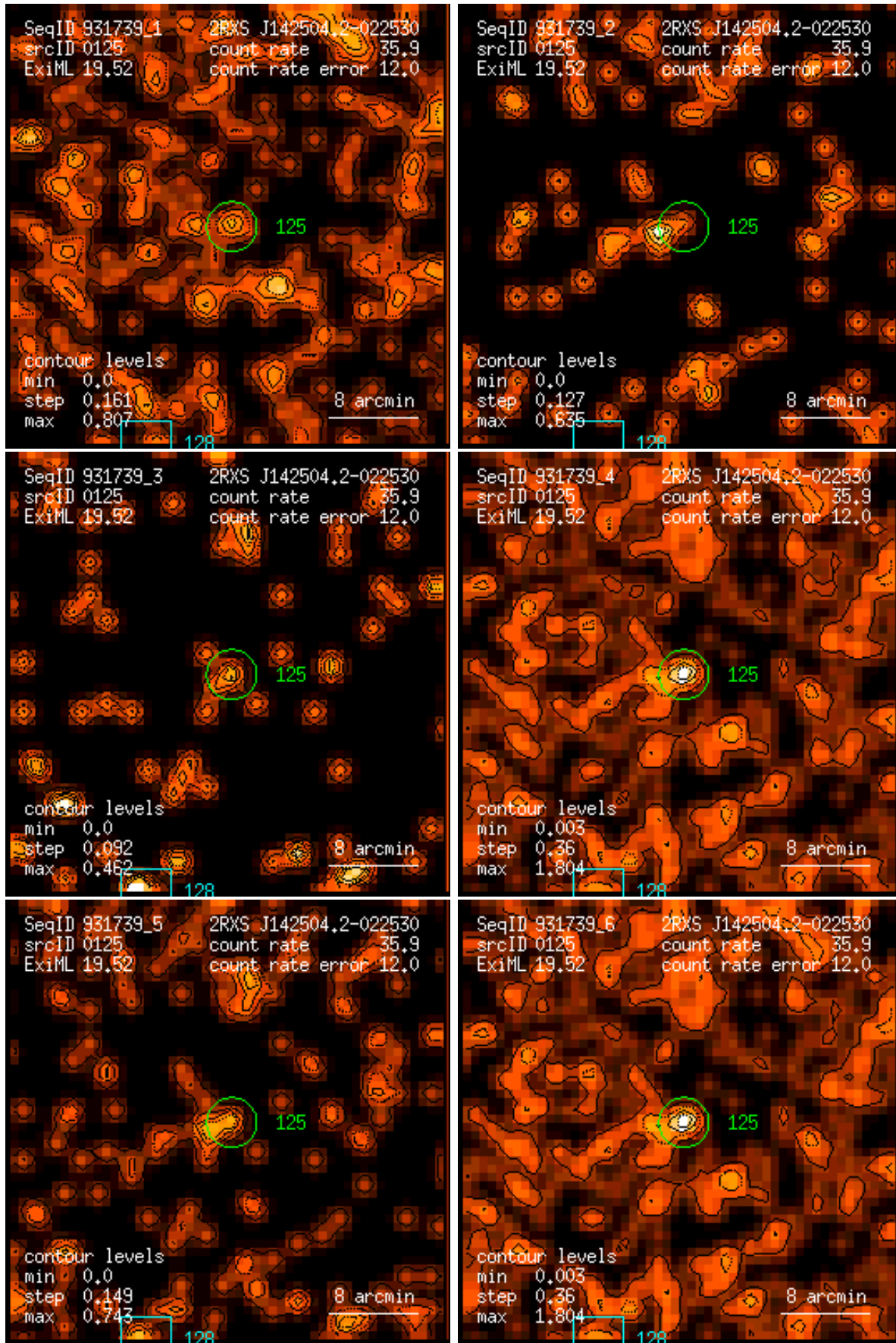
Figure 125: RASS 931739: detection 0125: band rate images, Gaussian filter: (1) PSPC channels 11 – 41, (2) 52 – 90, (3) 91 – 201, (4) 11 – 235, (5) 52 – 201, (6) 11 – 201. Broad band rates in counts/ks. Band rate contour levels in counts/ks/arcmin 2 .
