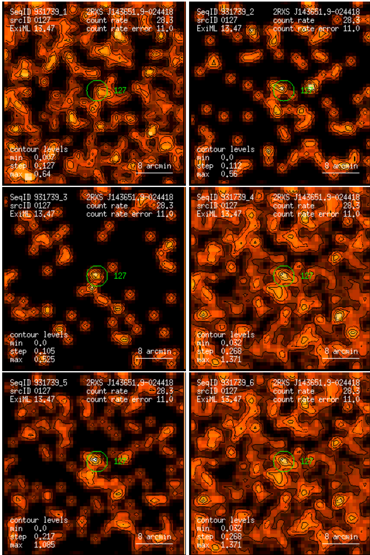
Figure 127: RASS 931739: detection 0127: band rate images, Gaussian filter: (1) PSPC channels 11 – 41, (2) 52 – 90, (3) 91 – 201, (4) 11 – 235, (5) 52 – 201, (6) 11 – 201. Broad band rates in counts/ks. Band rate contour levels in counts/ks/arcmin 2 .
