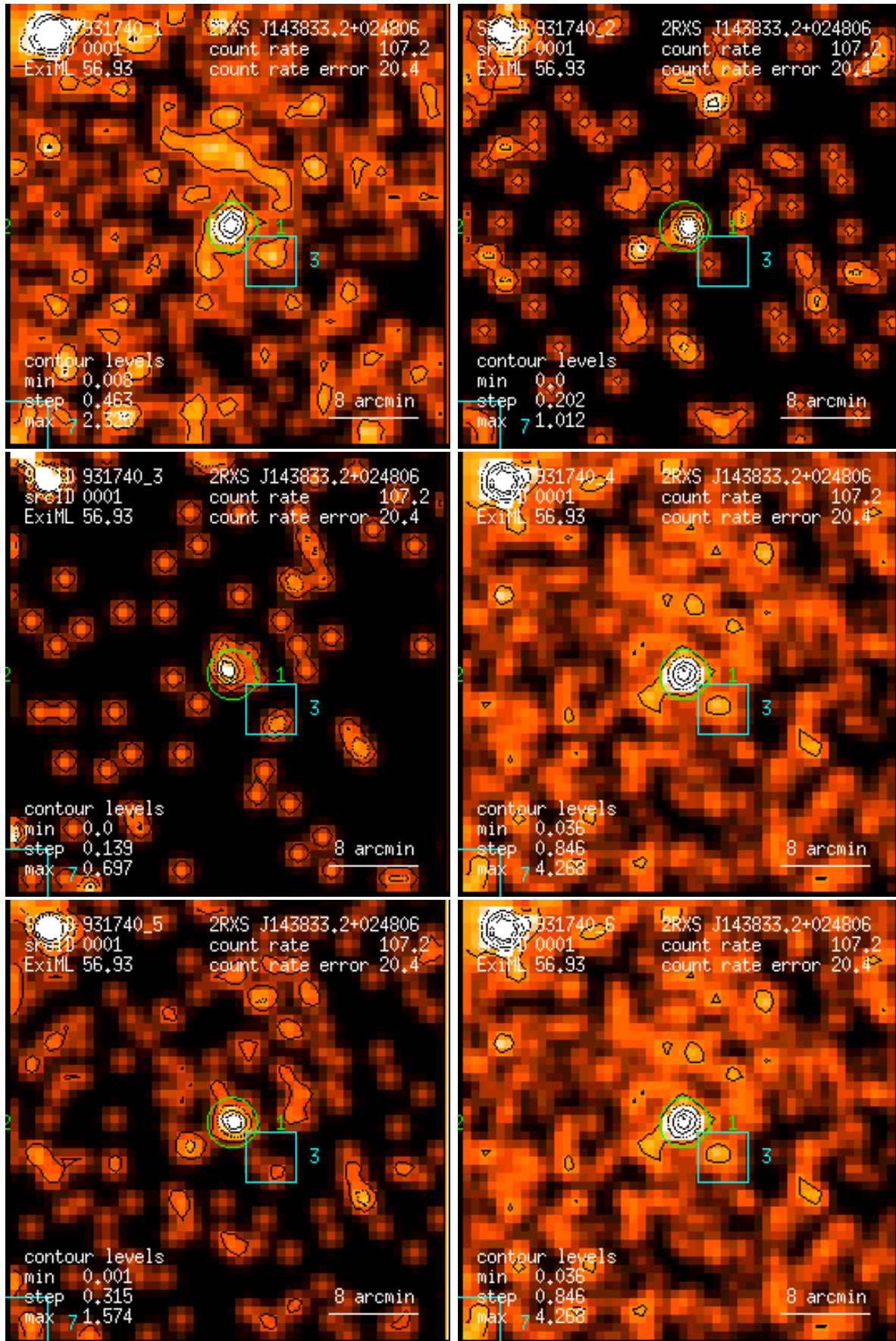
Figure 1: RASS 931740: detection 0001: band rate images, Gaussian filter: (1) PSPC channels 11 – 41, (2) 52 – 90, (3) 91 – 201, (4) 11 – 235, (5) 52 – 201, (6) 11 – 201. Broad band rates in counts/ks. Band rate contour levels in counts/ks/arcmin 2 .
