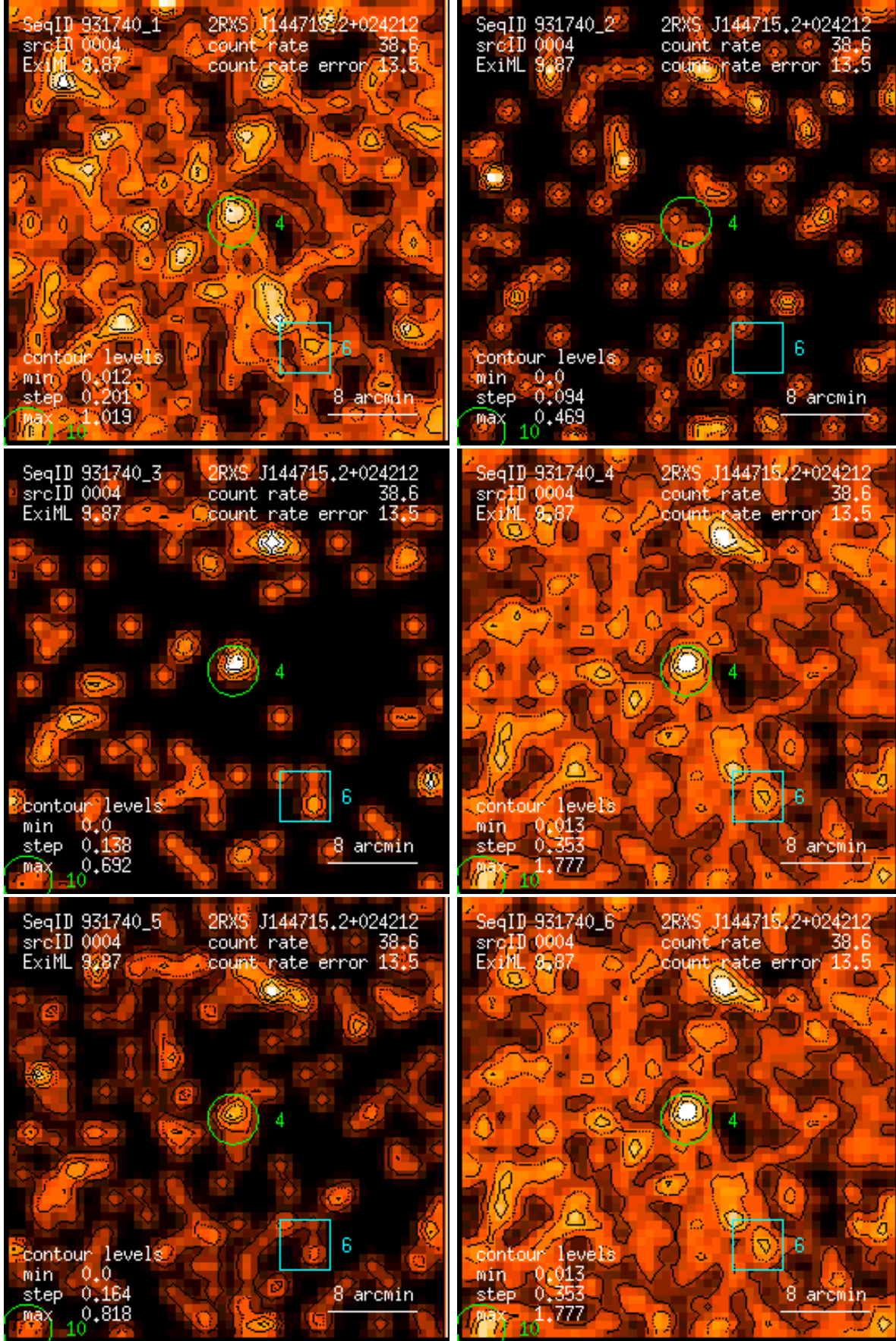
Figure 4: RASS 931740: detection 0004: band rate images, Gaussian filter: (1) PSPC channels 11 – 41, (2) 52 – 90, (3) 91 – 201, (4) 11 – 235, (5) 52 – 201, (6) 11 – 201. Broad band rates in counts/ks. Band rate contour levels in counts/ks/arcmin 2 .
