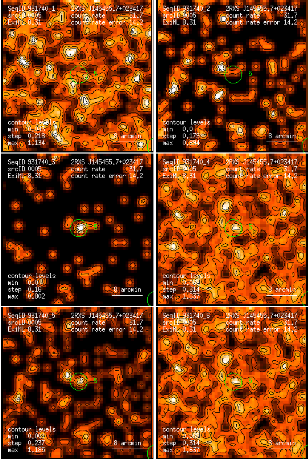
Figure 5: RASS 931740: detection 0005: band rate images, Gaussian filter: (1) PSPC channels 11 – 41, (2) 52 – 90, (3) 91 – 201, (4) 11 – 235, (5) 52 – 201, (6) 11 – 201. Broad band rates in counts/ks. Band rate contour levels in counts/ks/arcmin 2 .
