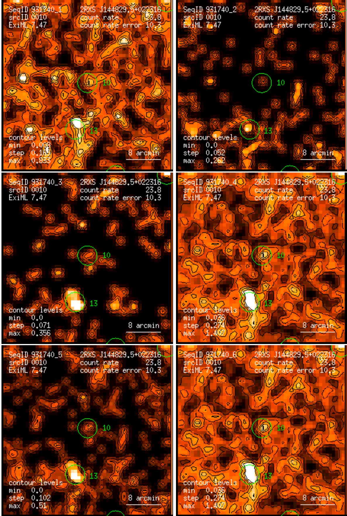
Figure 10: RASS 931740: detection 0010: band rate images, Gaussian filter: (1) PSPC channels 11 – 41, (2) 52 – 90, (3) 91 – 201, (4) 11 – 235, (5) 52 – 201, (6) 11 – 201. Broad band rates in counts/ks. Band rate contour levels in counts/ks/arcmin 2 .
