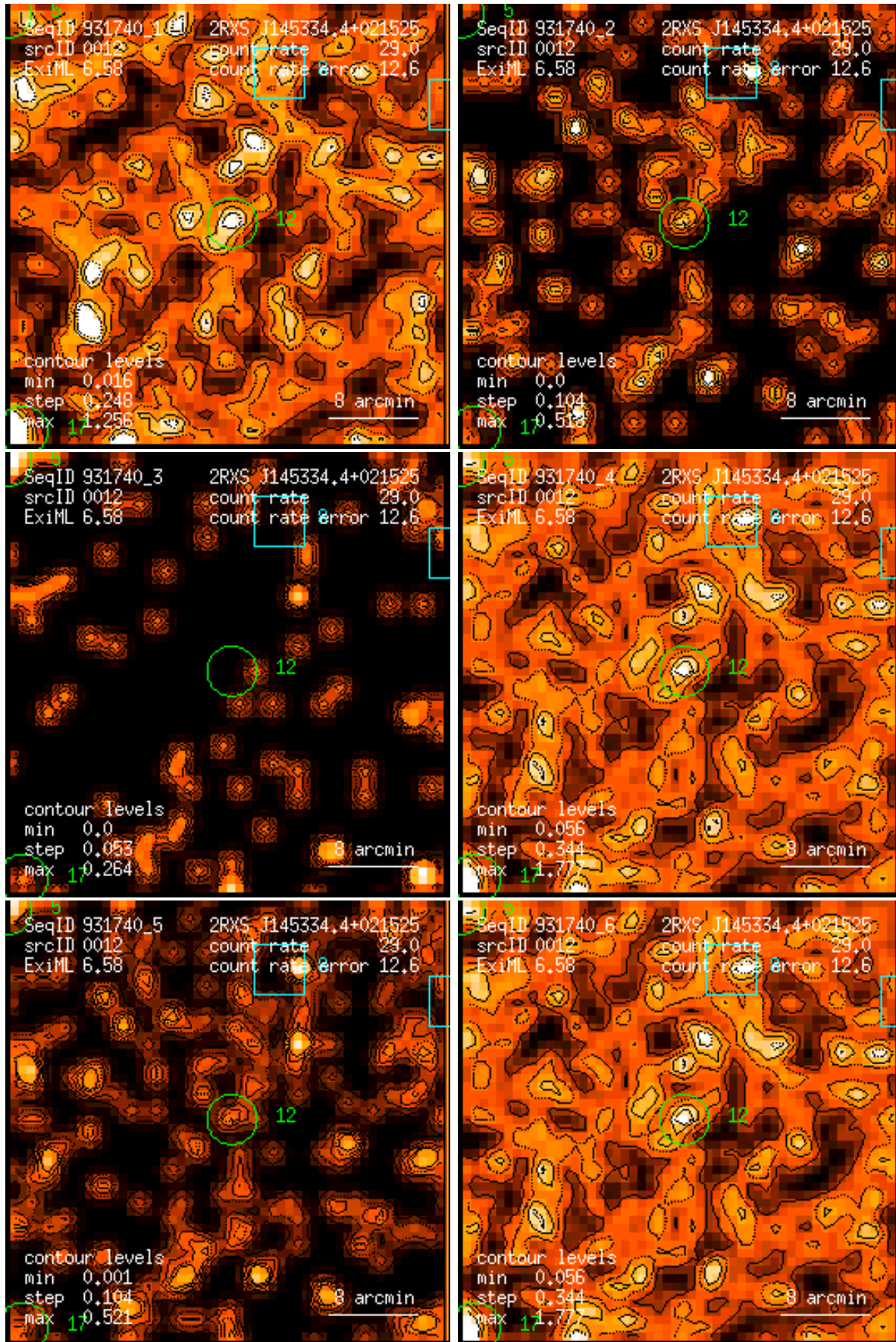
Figure 12: RASS 931740: detection 0012: band rate images, Gaussian filter: (1) PSPC channels 11 – 41, (2) 52 – 90, (3) 91 – 201, (4) 11 – 235, (5) 52 – 201, (6) 11 – 201. Broad band rates in counts/ks. Band rate contour levels in counts/ks/arcmin 2 .
