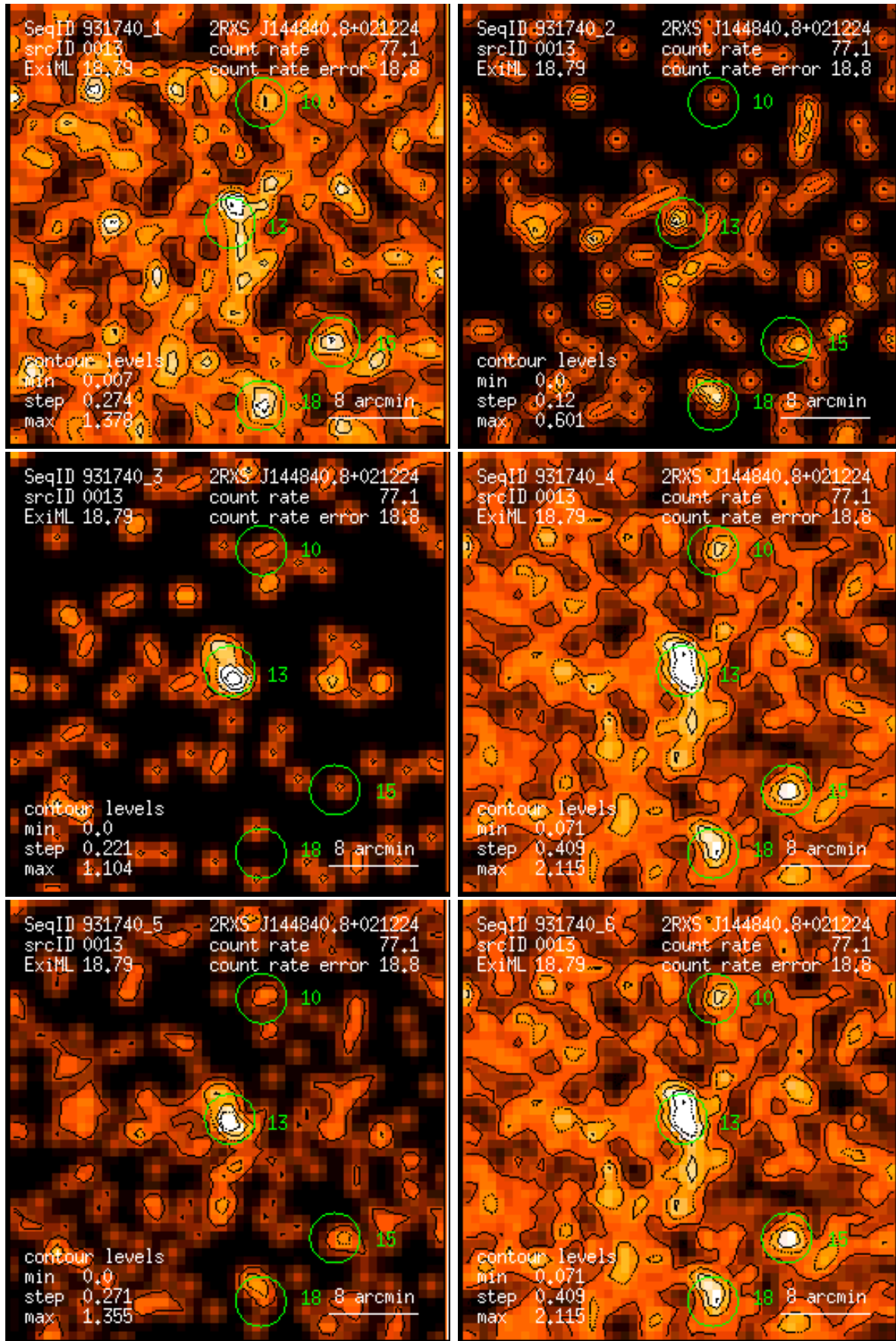
Figure 13: RASS 931740: detection 0013: band rate images, Gaussian filter: (1) PSPC channels 11 – 41, (2) 52 – 90, (3) 91 – 201, (4) 11 – 235, (5) 52 – 201, (6) 11 – 201. Broad band rates in counts/ks. Band rate contour levels in counts/ks/arcmin 2 .
