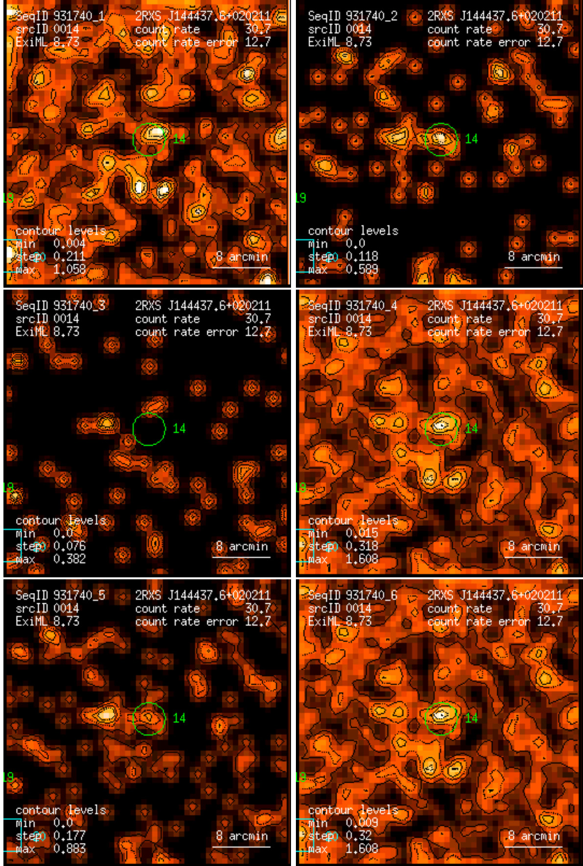
Figure 14: RASS 931740: detection 0014: band rate images, Gaussian filter: (1) PSPC channels 11 – 41, (2) 52 – 90, (3) 91 – 201, (4) 11 – 235, (5) 52 – 201, (6) 11 – 201. Broad band rates in counts/ks. Band rate contour levels in counts/ks/arcmin 2 .
