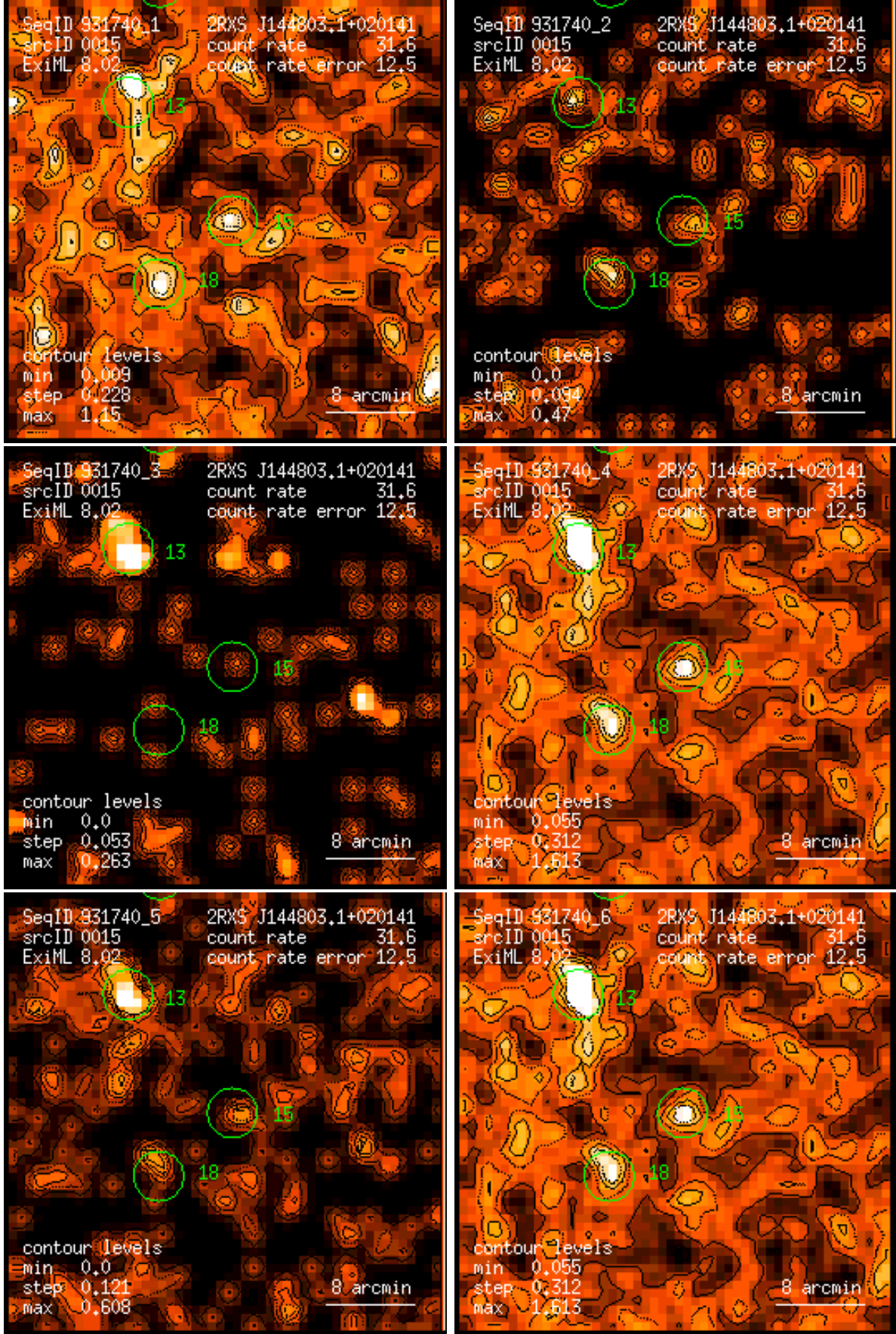
Figure 15: RASS 931740: detection 0015: band rate images, Gaussian filter: (1) PSPC channels 11 – 41, (2) 52 – 90, (3) 91 – 201, (4) 11 – 235, (5) 52 – 201, (6) 11 – 201. Broad band rates in counts/ks. Band rate contour levels in counts/ks/arcmin 2 .
