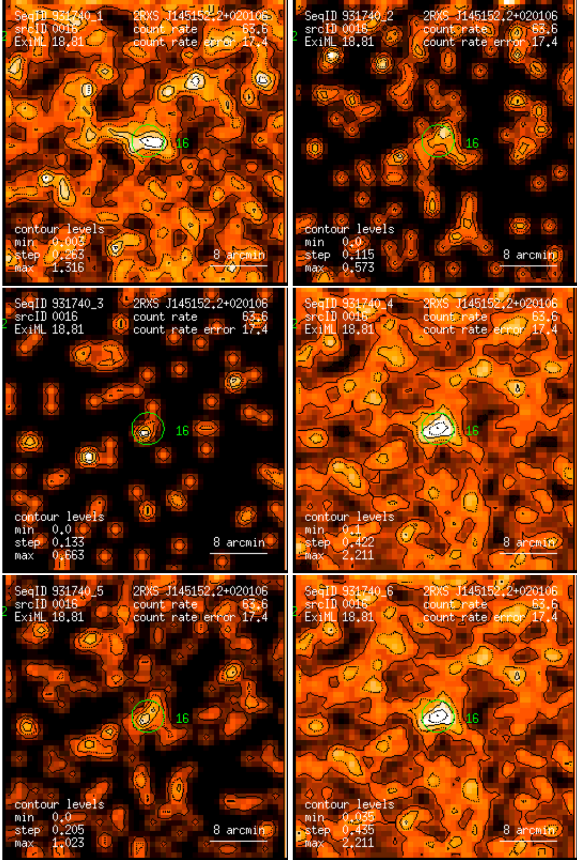
Figure 16: RASS 931740: detection 0016: band rate images, Gaussian filter: (1) PSPC channels 11 – 41, (2) 52 – 90, (3) 91 – 201, (4) 11 – 235, (5) 52 – 201, (6) 11 – 201. Broad band rates in counts/ks. Band rate contour levels in counts/ks/arcmin 2 .
