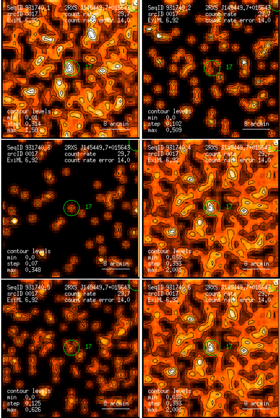
Figure 17: RASS 931740: detection 0017: band rate images, Gaussian filter: (1) PSPC channels 11 – 41, (2) 52 – 90, (3) 91 – 201, (4) 11 – 235, (5) 52 – 201, (6) 11 – 201. Broad band rates in counts/ks. Band rate contour levels in counts/ks/arcmin 2 .
