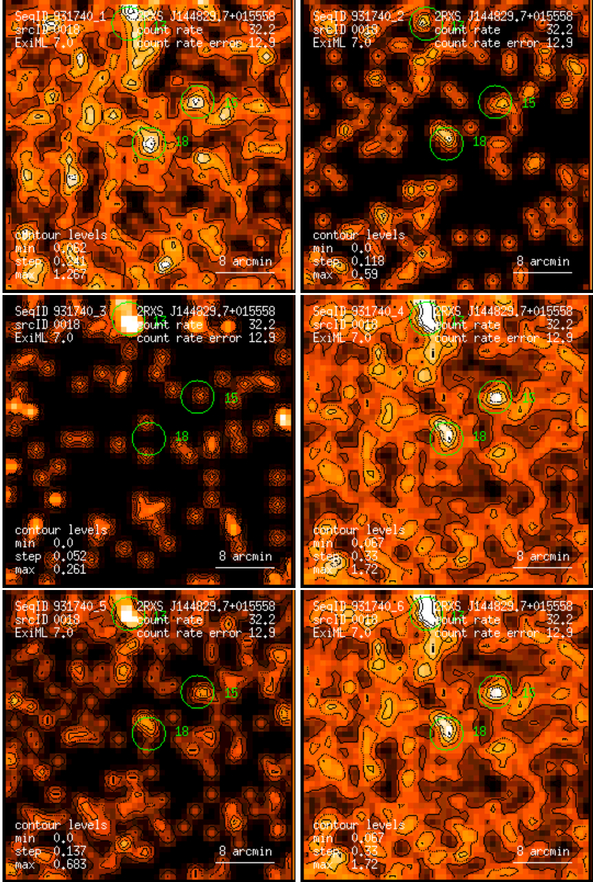
Figure 18: RASS 931740: detection 0018: band rate images, Gaussian filter: (1) PSPC channels 11 – 41, (2) 52 – 90, (3) 91 – 201, (4) 11 – 235, (5) 52 – 201, (6) 11 – 201. Broad band rates in counts/ks. Band rate contour levels in counts/ks/arcmin 2 .
