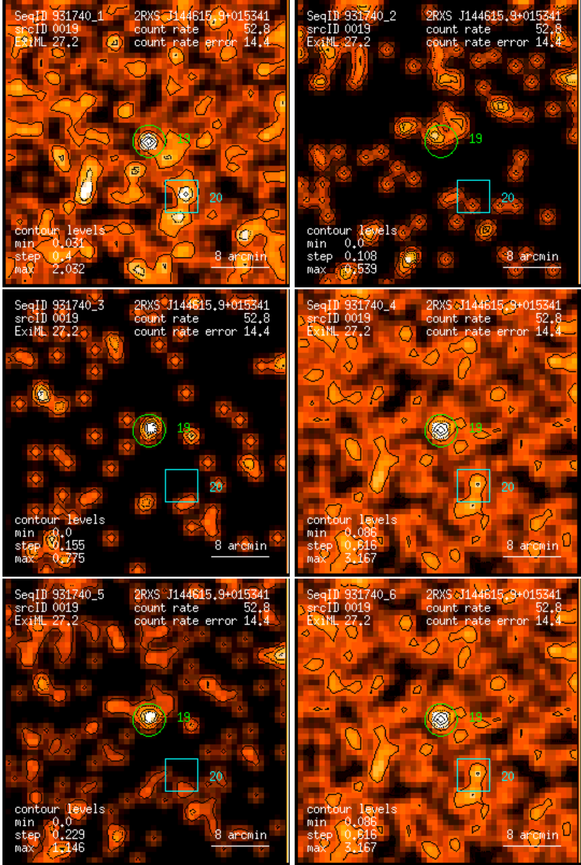
Figure 19: RASS 931740: detection 0019: band rate images, Gaussian filter: (1) PSPC channels 11 – 41, (2) 52 – 90, (3) 91 – 201, (4) 11 – 235, (5) 52 – 201, (6) 11 – 201. Broad band rates in counts/ks. Band rate contour levels in counts/ks/arcmin 2 .
