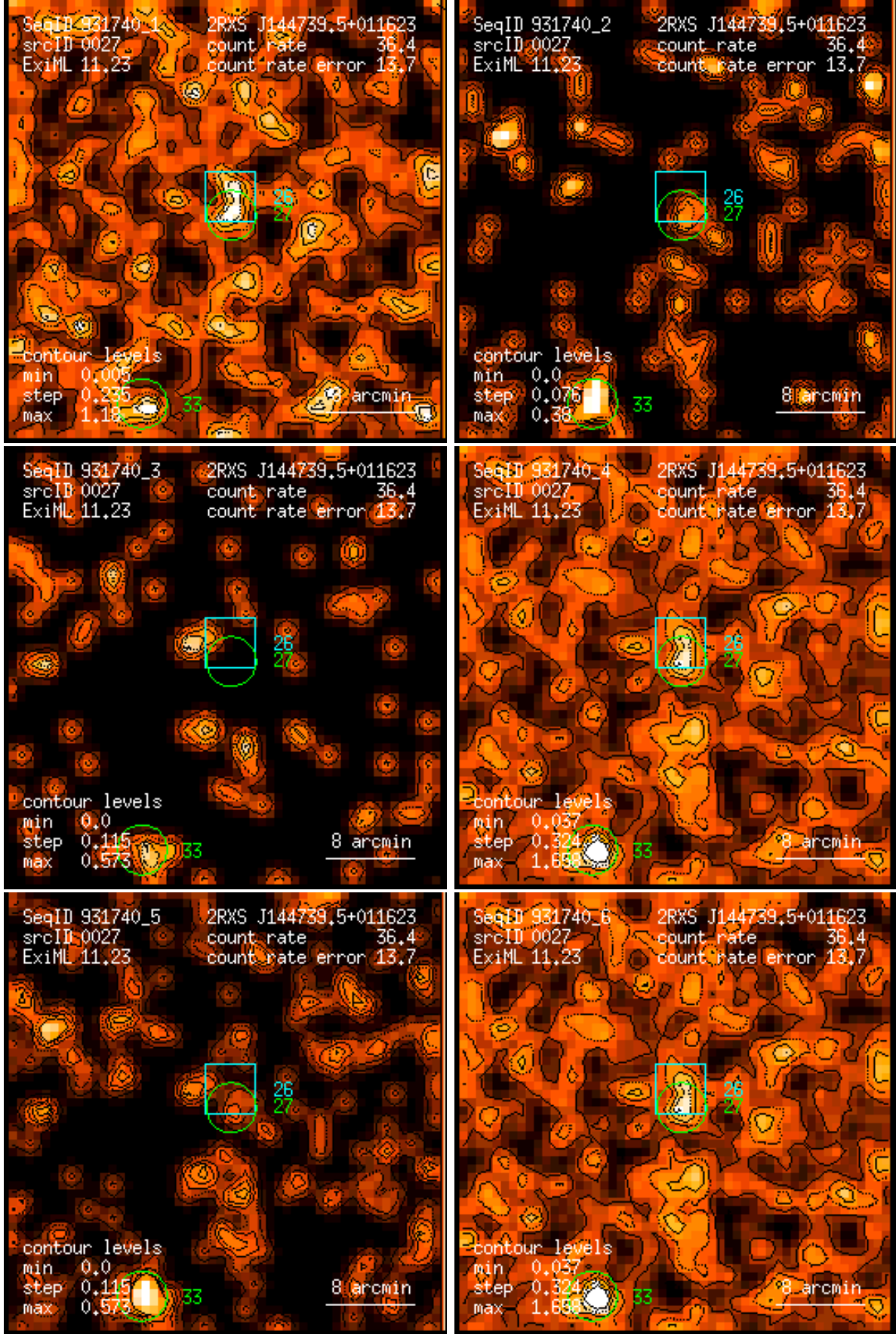
Figure 27: RASS 931740: detection 0027: band rate images, Gaussian filter: (1) PSPC channels 11 – 41, (2) 52 – 90, (3) 91 – 201, (4) 11 – 235, (5) 52 – 201, (6) 11 – 201. Broad band rates in counts/ks. Band rate contour levels in counts/ks/arcmin 2 .
