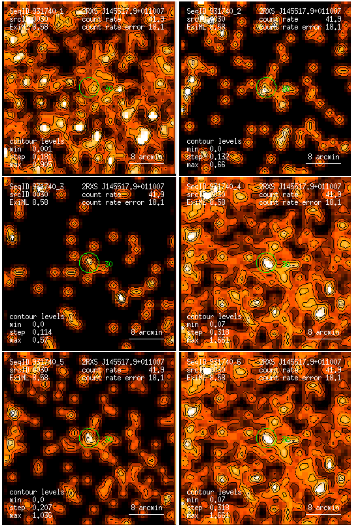
Figure 30: RASS 931740: detection 0030: band rate images, Gaussian filter: (1) PSPC channels 11 – 41, (2) 52 – 90, (3) 91 – 201, (4) 11 – 235, (5) 52 – 201, (6) 11 – 201. Broad band rates in counts/ks. Band rate contour levels in counts/ks/arcmin 2 .
