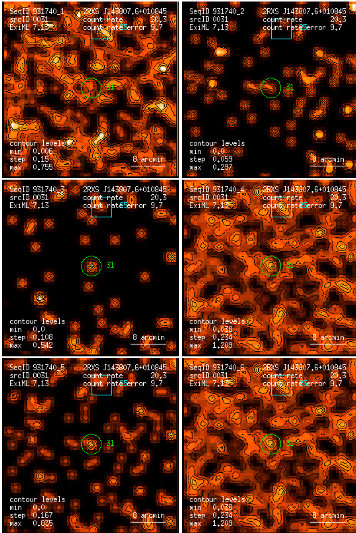
Figure 31: RASS 931740: detection 0031: band rate images, Gaussian filter: (1) PSPC channels 11 – 41, (2) 52 – 90, (3) 91 – 201, (4) 11 – 235, (5) 52 – 201, (6) 11 – 201. Broad band rates in counts/ks. Band rate contour levels in counts/ks/arcmin 2 .
