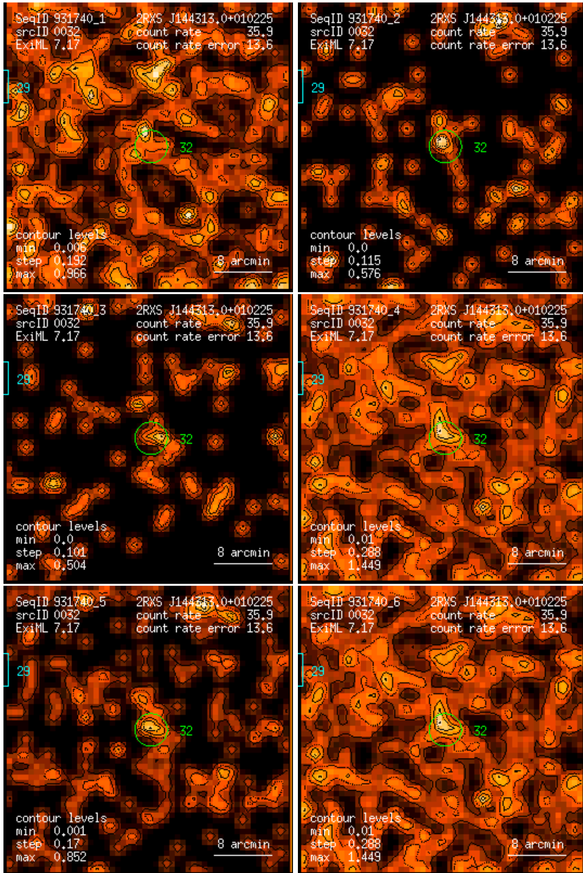
Figure 32: RASS 931740: detection 0032: band rate images, Gaussian filter: (1) PSPC channels 11 – 41, (2) 52 – 90, (3) 91 – 201, (4) 11 – 235, (5) 52 – 201, (6) 11 – 201. Broad band rates in counts/ks. Band rate contour levels in counts/ks/arcmin 2 .
