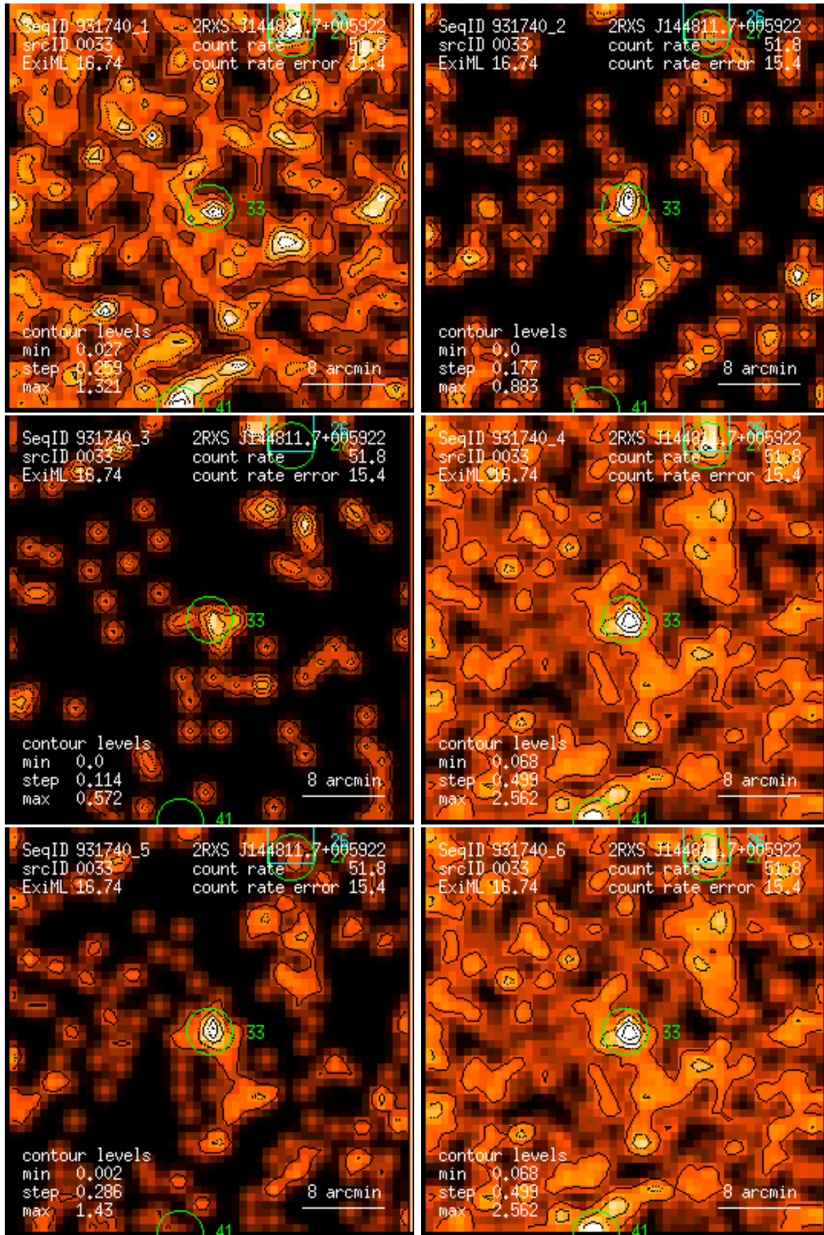
Figure 33: RASS 931740: detection 0033: band rate images, Gaussian filter: (1) PSPC channels 11 – 41, (2) 52 – 90, (3) 91 – 201, (4) 11 – 235, (5) 52 – 201, (6) 11 – 201. Broad band rates in counts/ks. Band rate contour levels in counts/ks/arcmin 2 .
