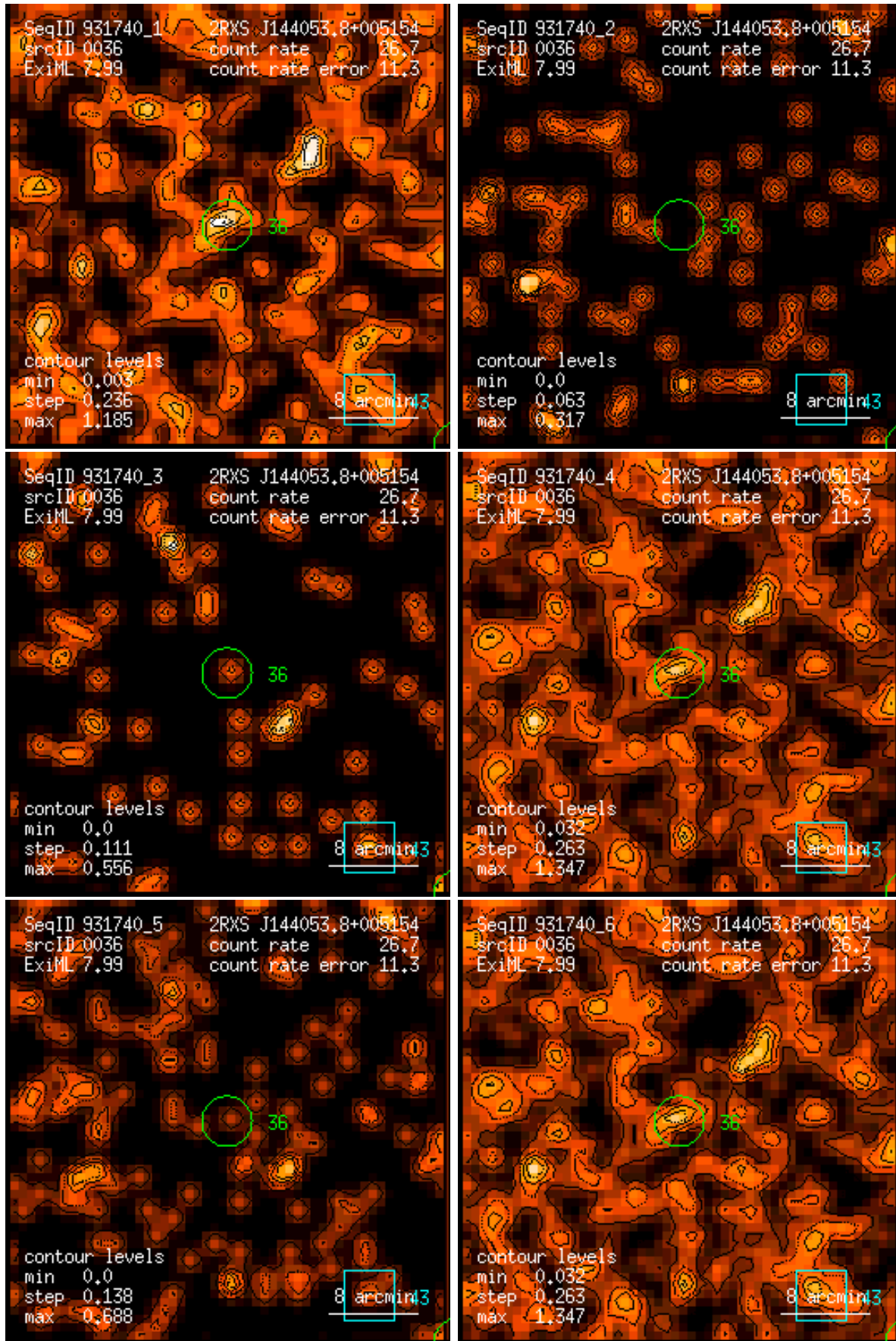
Figure 36: RASS 931740: detection 0036: band rate images, Gaussian filter: (1) PSPC channels 11 – 41, (2) 52 – 90, (3) 91 – 201, (4) 11 – 235, (5) 52 – 201, (6) 11 – 201. Broad band rates in counts/ks. Band rate contour levels in counts/ks/arcmin 2 .
