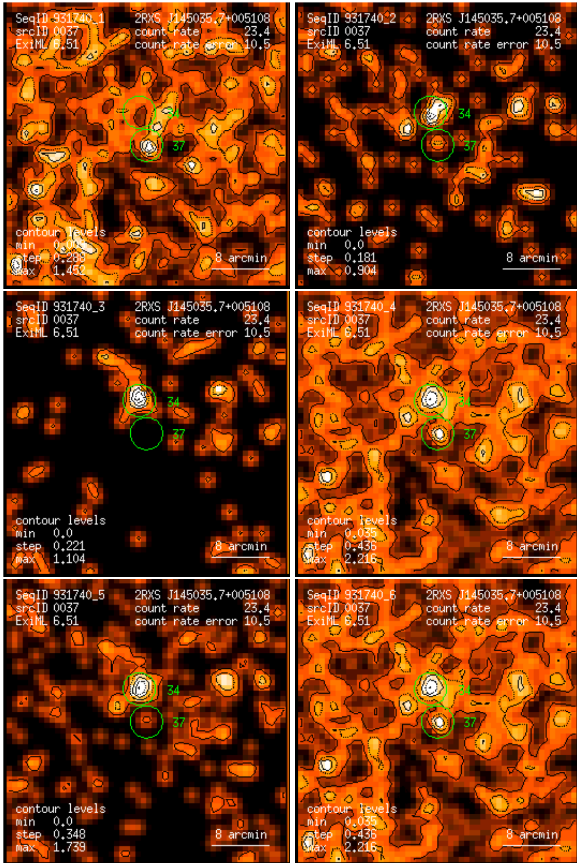
Figure 37: RASS 931740: detection 0037: band rate images, Gaussian filter: (1) PSPC channels 11 – 41, (2) 52 – 90, (3) 91 – 201, (4) 11 – 235, (5) 52 – 201, (6) 11 – 201. Broad band rates in counts/ks. Band rate contour levels in counts/ks/arcmin 2 .
