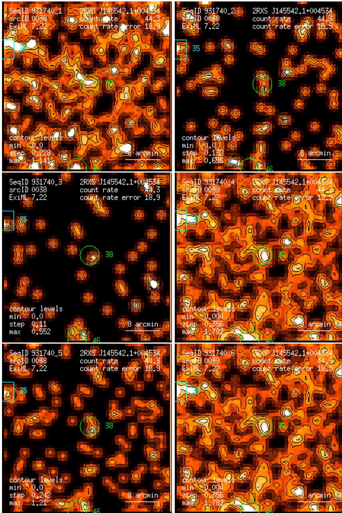
Figure 38: RASS 931740: detection 0038: band rate images, Gaussian filter: (1) PSPC channels 11 – 41, (2) 52 – 90, (3) 91 – 201, (4) 11 – 235, (5) 52 – 201, (6) 11 – 201. Broad band rates in counts/ks. Band rate contour levels in counts/ks/arcmin 2 .
