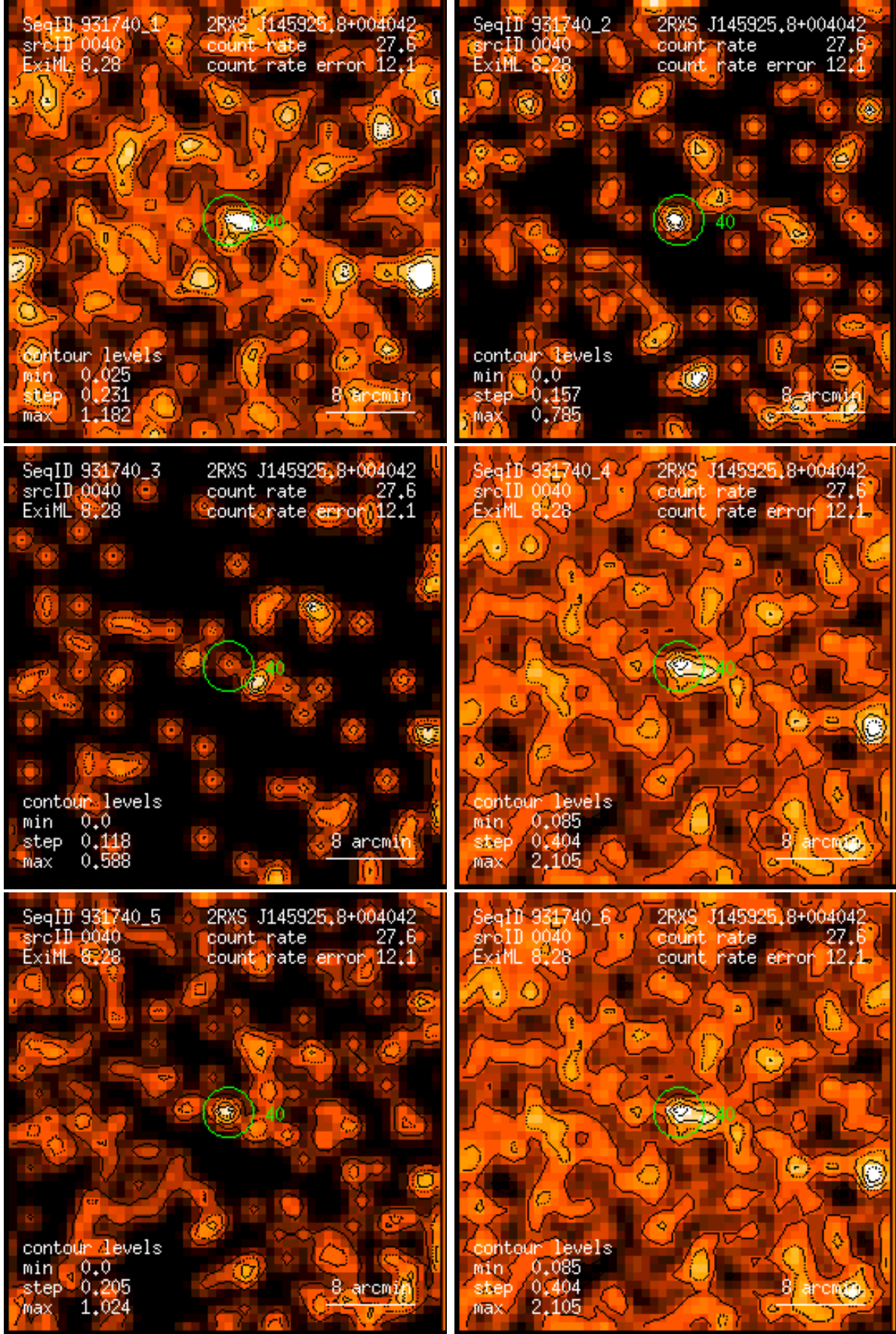
Figure 40: RASS 931740: detection 0040: band rate images, Gaussian filter: (1) PSPC channels 11 – 41, (2) 52 – 90, (3) 91 – 201, (4) 11 – 235, (5) 52 – 201, (6) 11 – 201. Broad band rates in counts/ks. Band rate contour levels in counts/ks/arcmin 2 .
