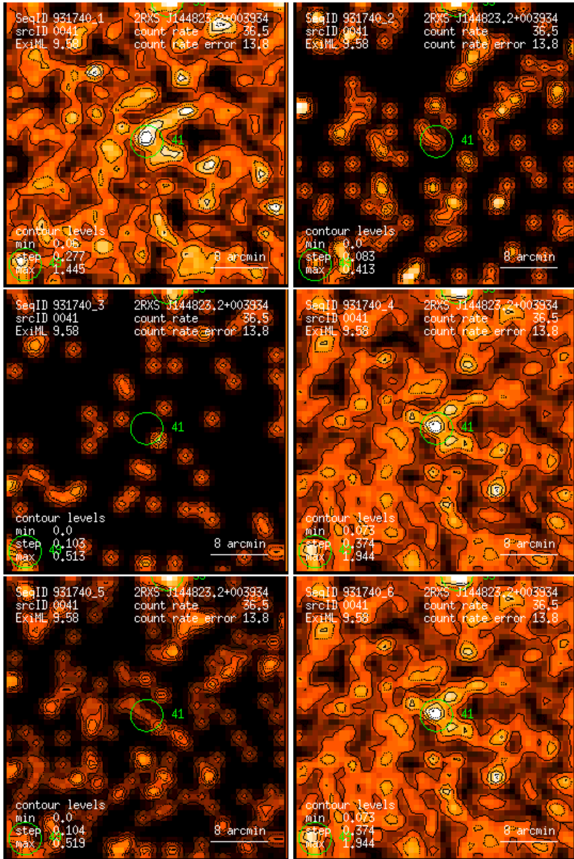
Figure 41: RASS 931740: detection 0041: band rate images, Gaussian filter: (1) PSPC channels 11 – 41, (2) 52 – 90, (3) 91 – 201, (4) 11 – 235, (5) 52 – 201, (6) 11 – 201. Broad band rates in counts/ks. Band rate contour levels in counts/ks/arcmin 2 .
