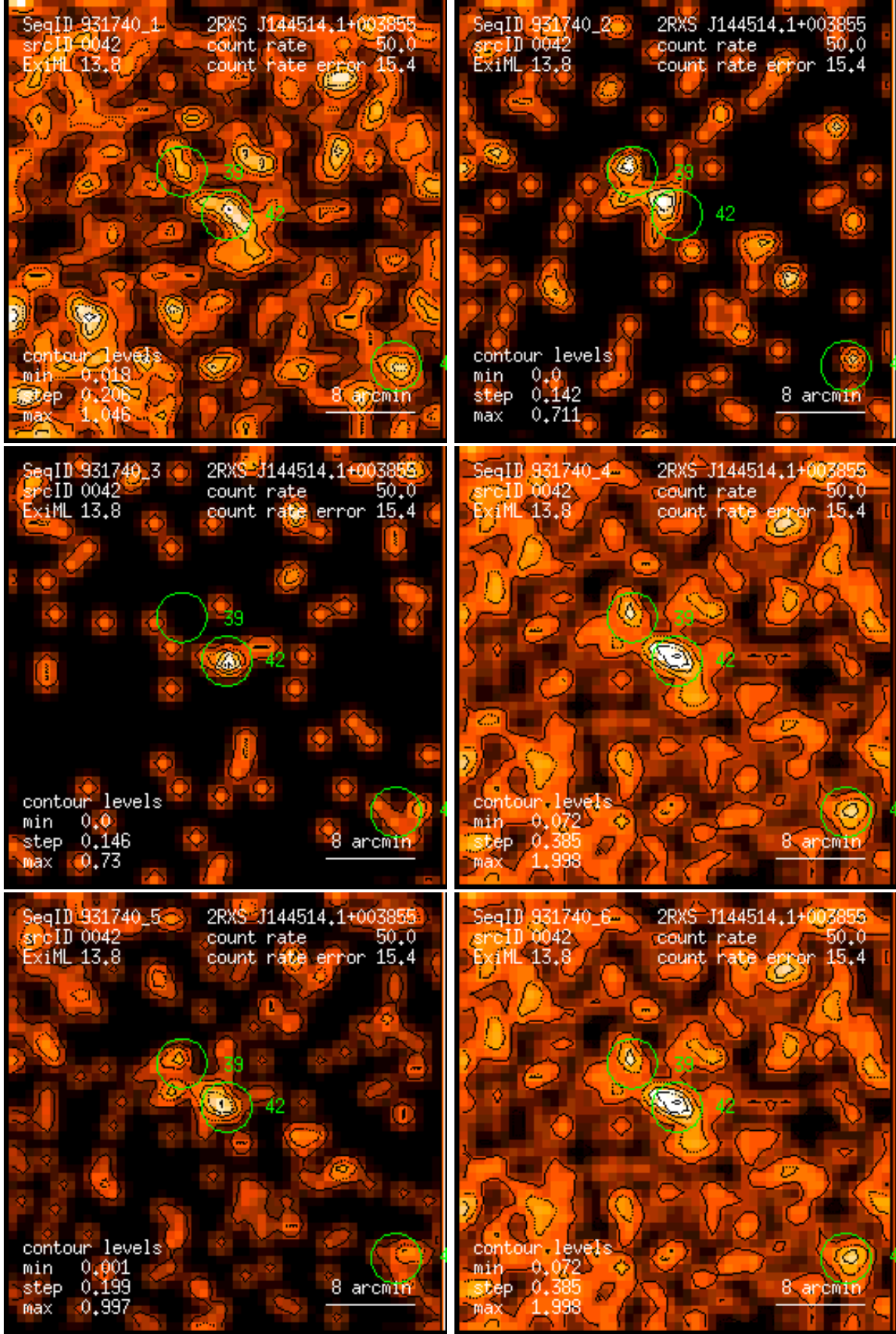
Figure 42: RASS 931740: detection 0042: band rate images, Gaussian filter: (1) PSPC channels 11 – 41, (2) 52 – 90, (3) 91 – 201, (4) 11 – 235, (5) 52 – 201, (6) 11 – 201. Broad band rates in counts/ks. Band rate contour levels in counts/ks/arcmin 2 .
