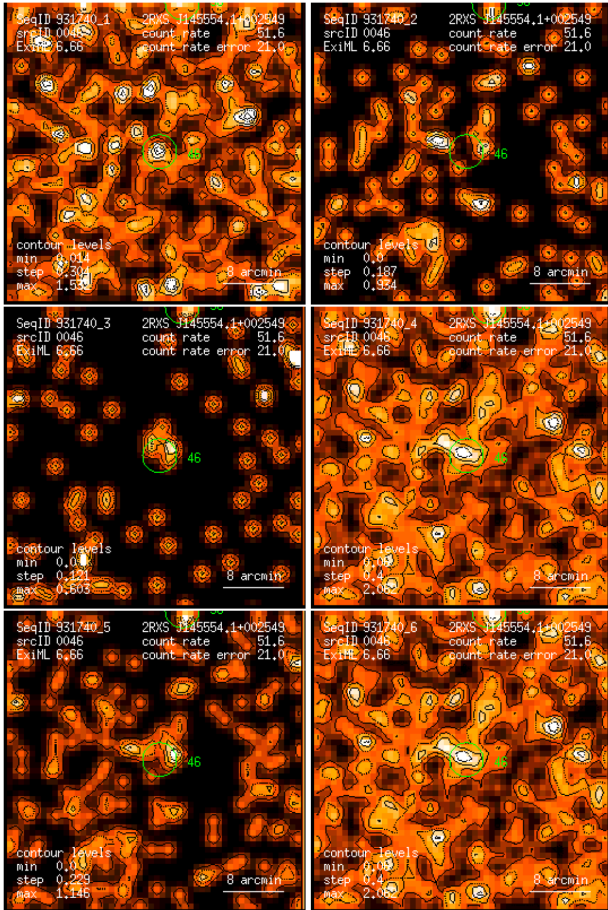
Figure 46: RASS 931740: detection 0046: band rate images, Gaussian filter: (1) PSPC channels 11 – 41, (2) 52 – 90, (3) 91 – 201, (4) 11 – 235, (5) 52 – 201, (6) 11 – 201. Broad band rates in counts/ks. Band rate contour levels in counts/ks/arcmin 2 .
