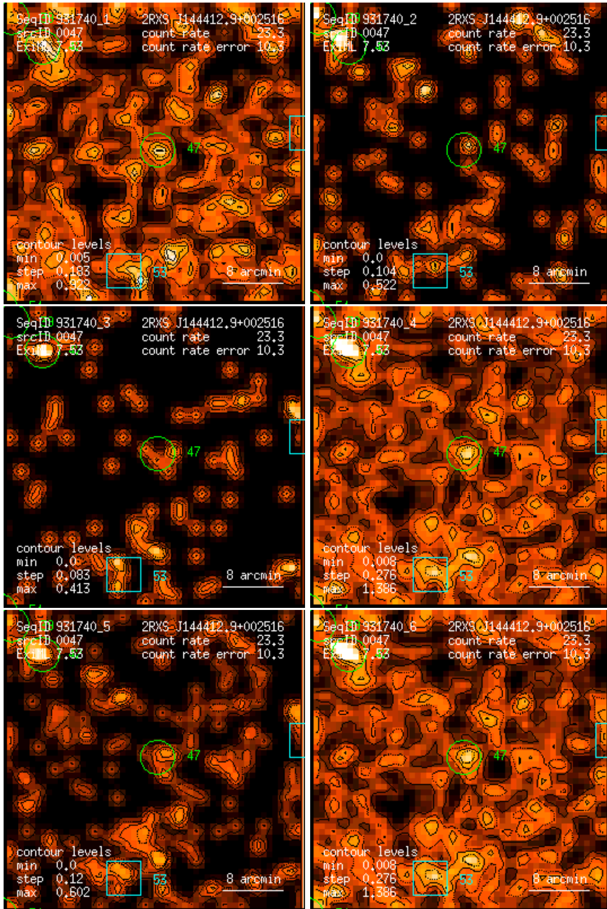
Figure 47: RASS 931740: detection 0047: band rate images, Gaussian filter: (1) PSPC channels 11 – 41, (2) 52 – 90, (3) 91 – 201, (4) 11 – 235, (5) 52 – 201, (6) 11 – 201. Broad band rates in counts/ks. Band rate contour levels in counts/ks/arcmin 2 .
