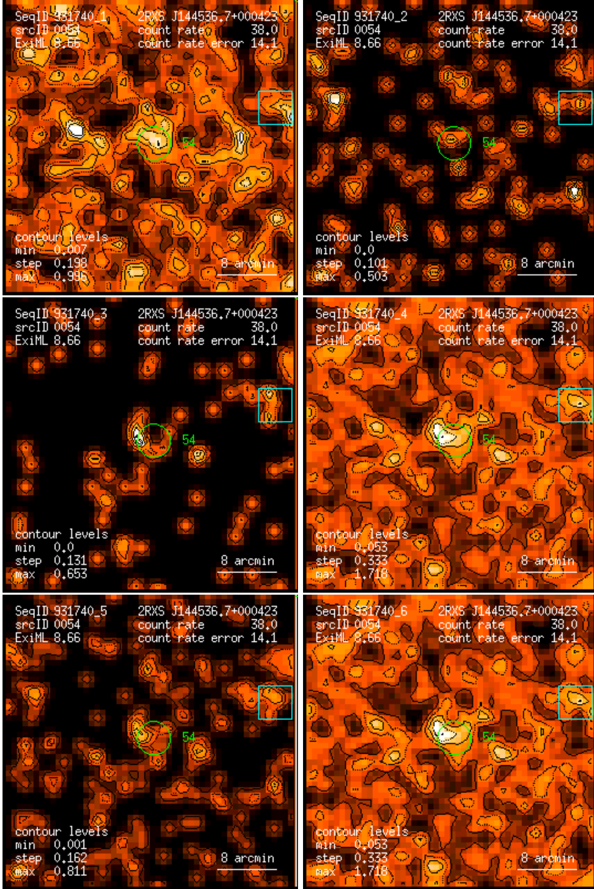
Figure 54: RASS 931740: detection 0054: band rate images, Gaussian filter: (1) PSPC channels 11 – 41, (2) 52 – 90, (3) 91 – 201, (4) 11 – 235, (5) 52 – 201, (6) 11 – 201. Broad band rates in counts/ks. Band rate contour levels in counts/ks/arcmin 2 .
