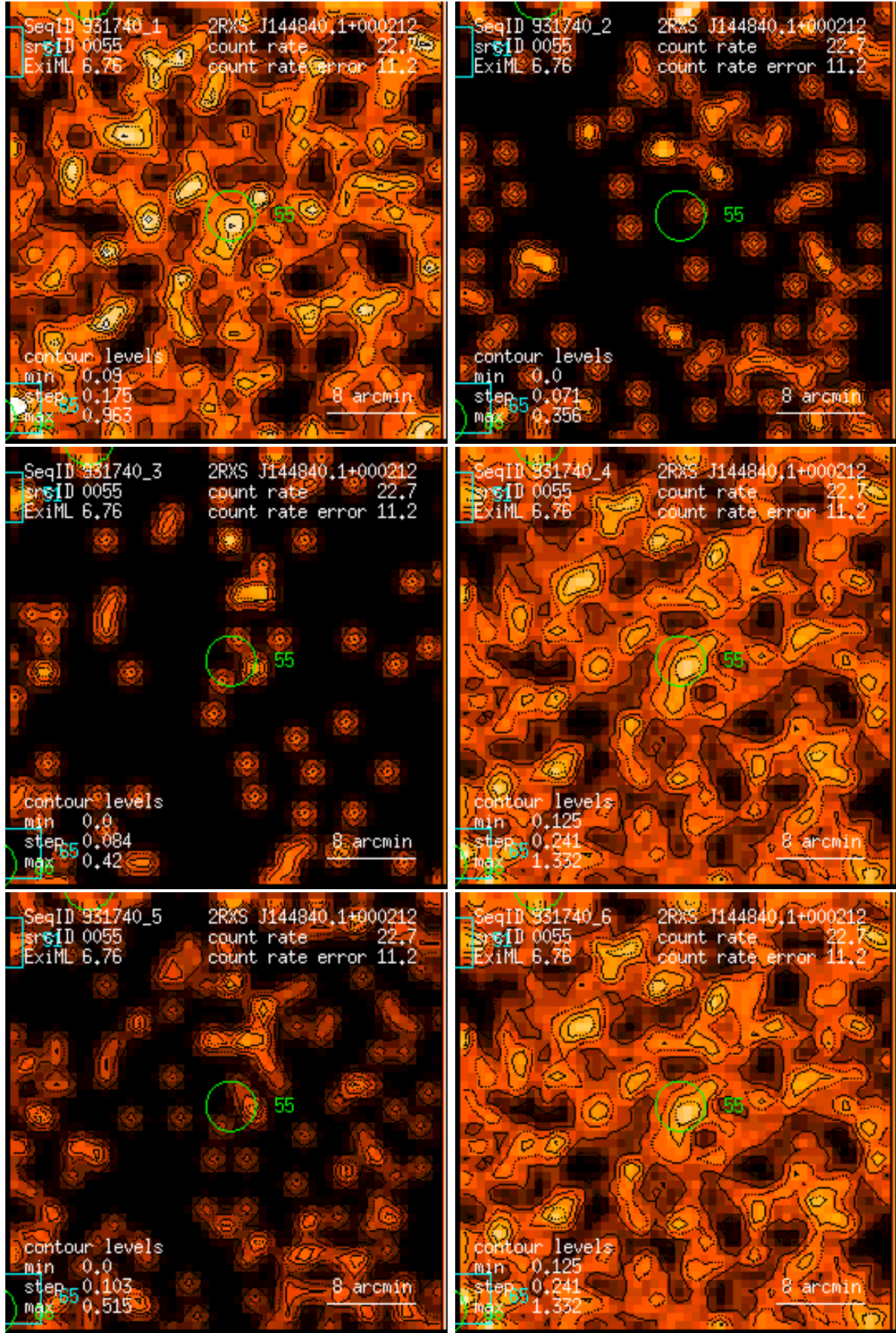
Figure 55: RASS 931740: detection 0055: band rate images, Gaussian filter: (1) PSPC channels 11 – 41, (2) 52 – 90, (3) 91 – 201, (4) 11 – 235, (5) 52 – 201, (6) 11 – 201. Broad band rates in counts/ks. Band rate contour levels in counts/ks/arcmin 2 .
