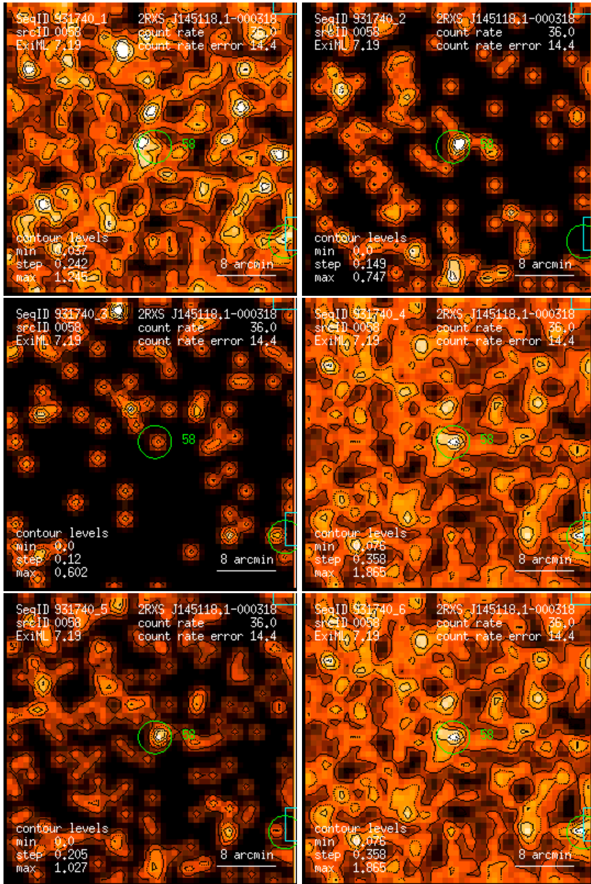
Figure 58: RASS 931740: detection 0058: band rate images, Gaussian filter: (1) PSPC channels 11 – 41, (2) 52 – 90, (3) 91 – 201, (4) 11 – 235, (5) 52 – 201, (6) 11 – 201. Broad band rates in counts/ks. Band rate contour levels in counts/ks/arcmin 2 .
