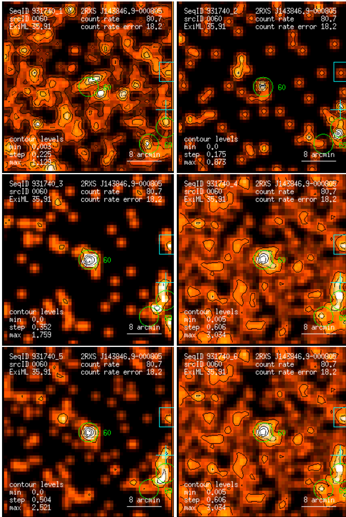
Figure 60: RASS 931740: detection 0060: band rate images, Gaussian filter: (1) PSPC channels 11 – 41, (2) 52 – 90, (3) 91 – 201, (4) 11 – 235, (5) 52 – 201, (6) 11 – 201. Broad band rates in counts/ks. Band rate contour levels in counts/ks/arcmin 2 .
