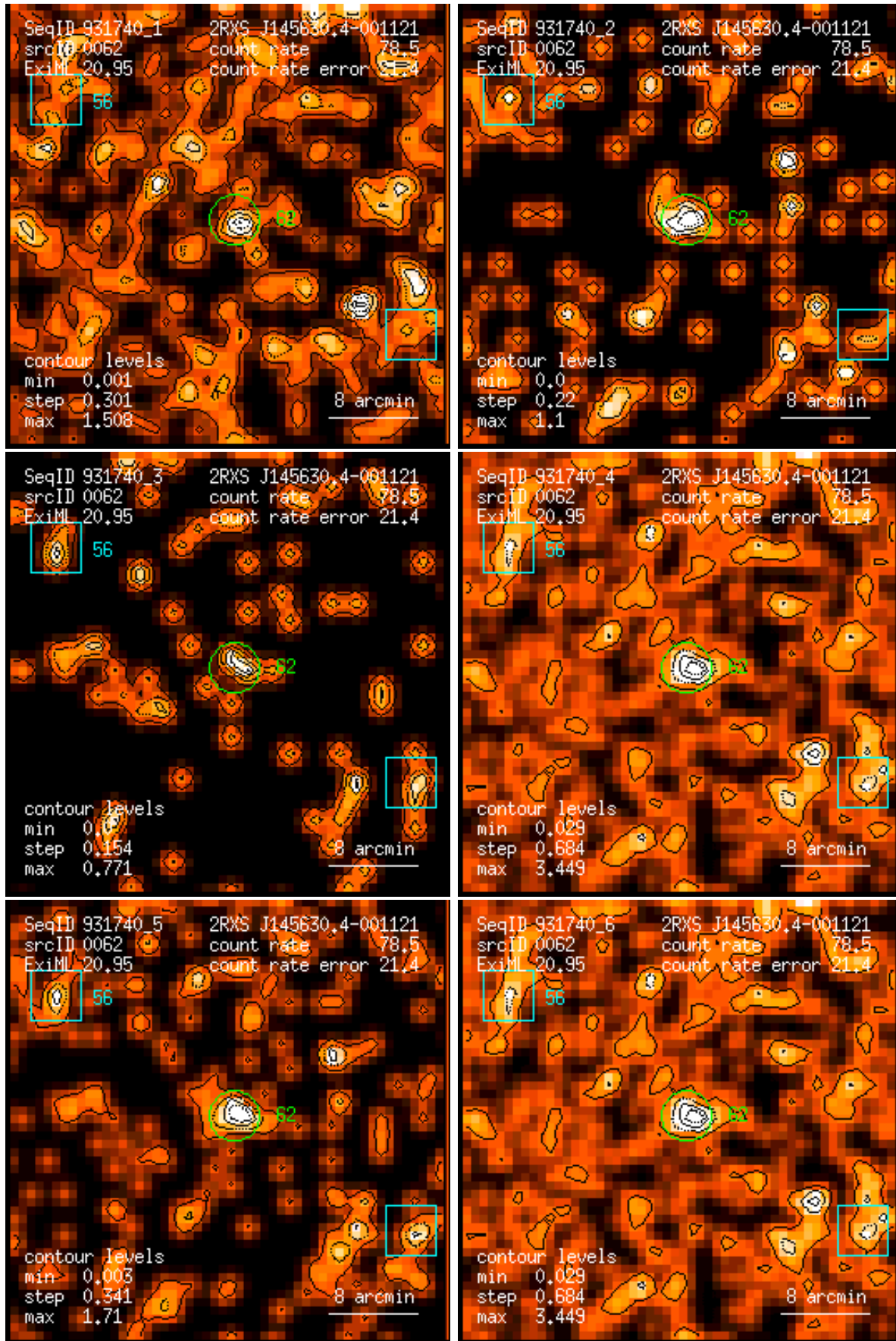
Figure 62: RASS 931740: detection 0062: band rate images, Gaussian filter: (1) PSPC channels 11 – 41, (2) 52 – 90, (3) 91 – 201, (4) 11 – 235, (5) 52 – 201, (6) 11 – 201. Broad band rates in counts/ks. Band rate contour levels in counts/ks/arcmin 2 .
