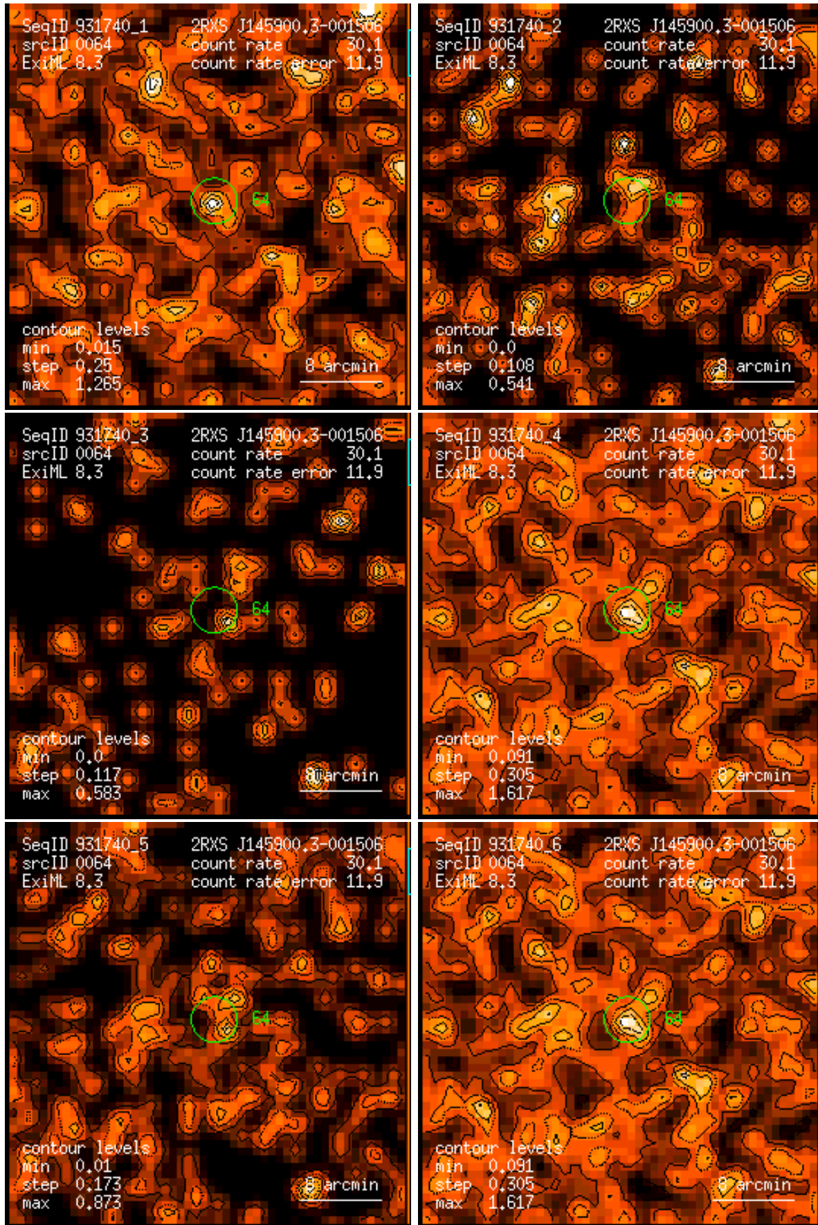
Figure 64: RASS 931740: detection 0064: band rate images, Gaussian filter: (1) PSPC channels 11 – 41, (2) 52 – 90, (3) 91 – 201, (4) 11 – 235, (5) 52 – 201, (6) 11 – 201. Broad band rates in counts/ks. Band rate contour levels in counts/ks/arcmin 2 .
