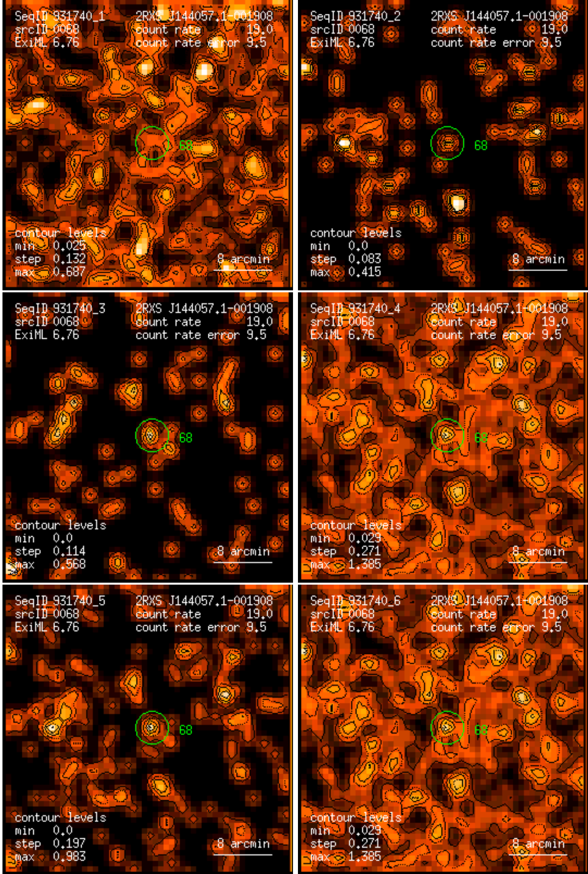
Figure 68: RASS 931740: detection 0068: band rate images, Gaussian filter: (1) PSPC channels 11 – 41, (2) 52 – 90, (3) 91 – 201, (4) 11 – 235, (5) 52 – 201, (6) 11 – 201. Broad band rates in counts/ks. Band rate contour levels in counts/ks/arcmin 2 .
