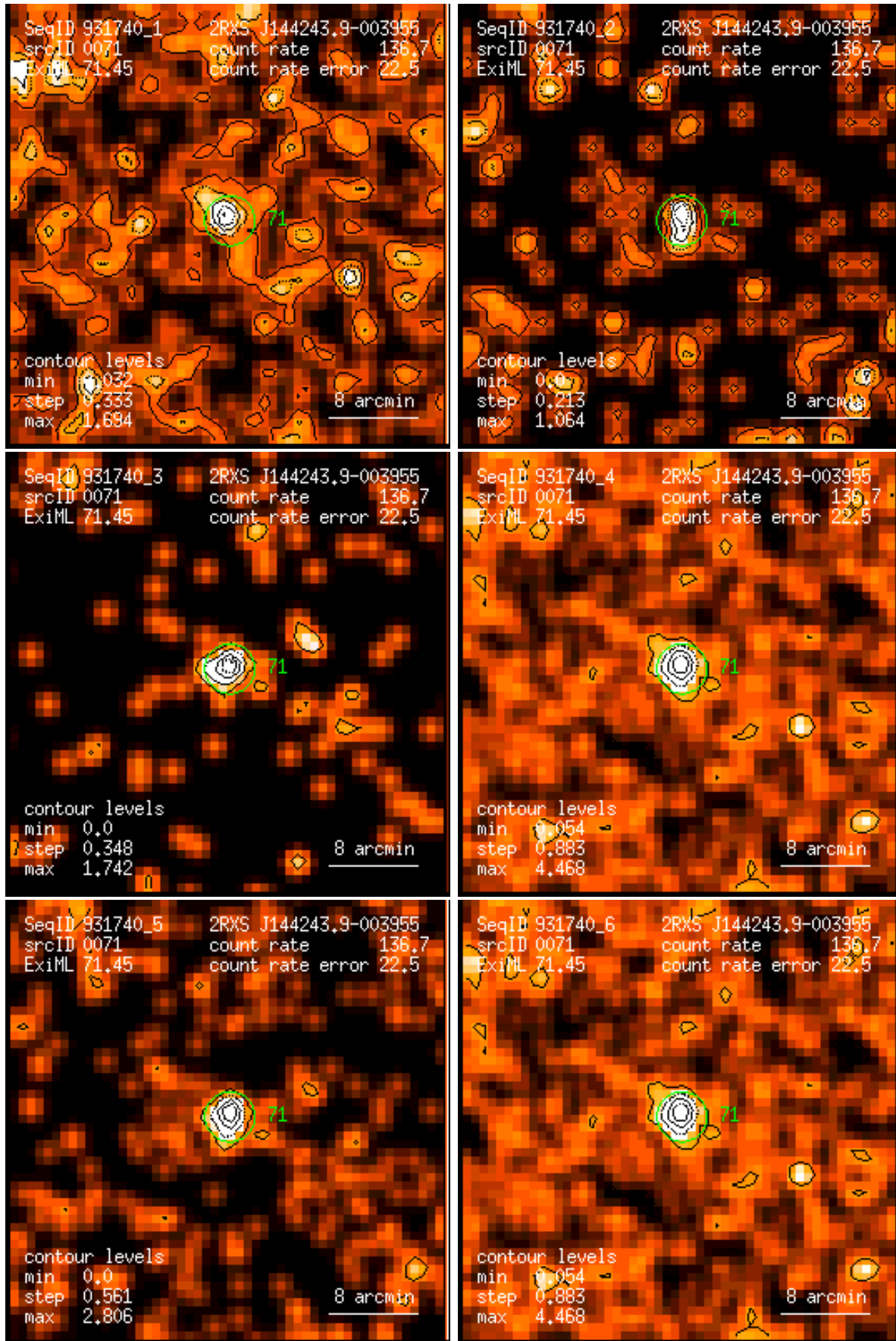
Figure 71: RASS 931740: detection 0071: band rate images, Gaussian filter: (1) PSPC channels 11 – 41, (2) 52 – 90, (3) 91 – 201, (4) 11 – 235, (5) 52 – 201, (6) 11 – 201. Broad band rates in counts/ks. Band rate contour levels in counts/ks/arcmin 2 .
