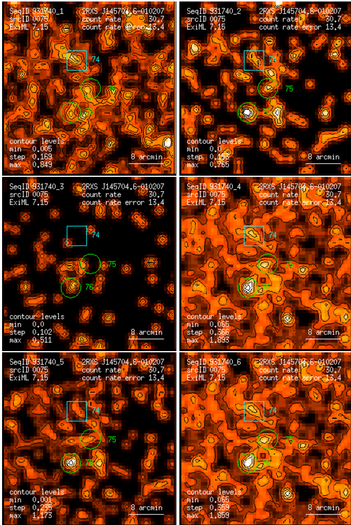
Figure 75: RASS 931740: detection 0075: band rate images, Gaussian filter: (1) PSPC channels 11 – 41, (2) 52 – 90, (3) 91 – 201, (4) 11 – 235, (5) 52 – 201, (6) 11 – 201. Broad band rates in counts/ks. Band rate contour levels in counts/ks/arcmin 2 .
