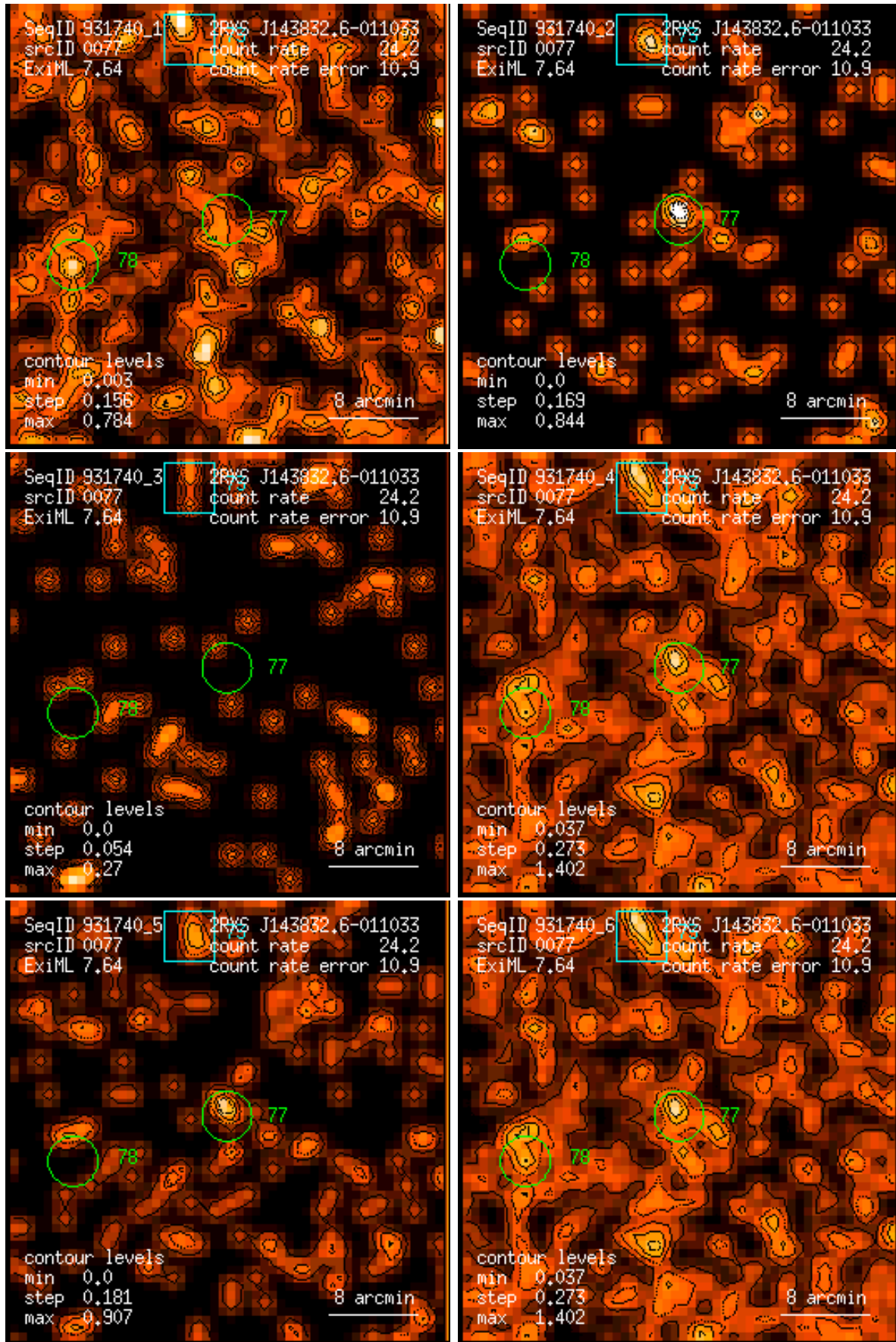
Figure 77: RASS 931740: detection 0077: band rate images, Gaussian filter: (1) PSPC channels 11 – 41, (2) 52 – 90, (3) 91 – 201, (4) 11 – 235, (5) 52 – 201, (6) 11 – 201. Broad band rates in counts/ks. Band rate contour levels in counts/ks/arcmin 2 .
