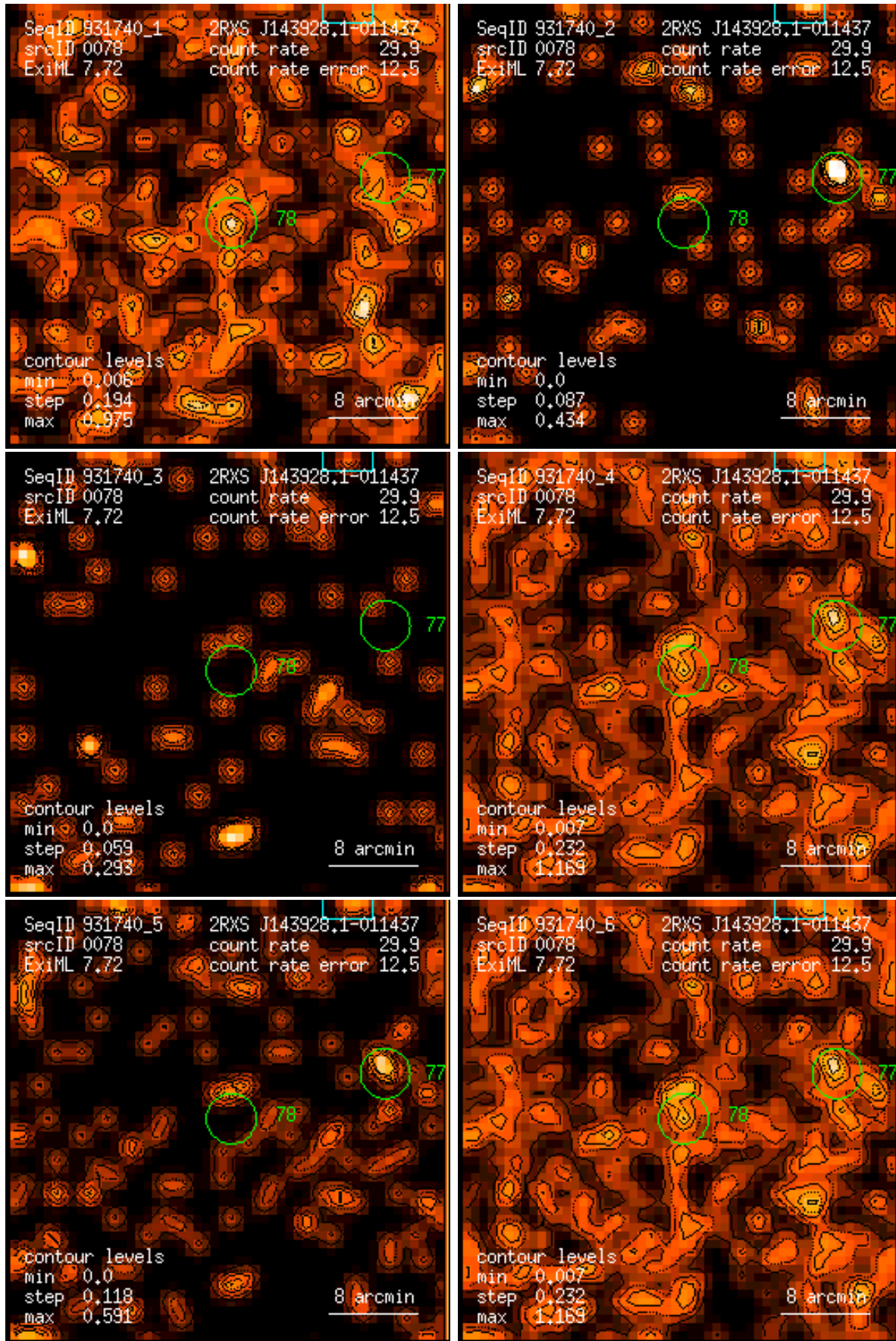
Figure 78: RASS 931740: detection 0078: band rate images, Gaussian filter: (1) PSPC channels 11 – 41, (2) 52 – 90, (3) 91 – 201, (4) 11 – 235, (5) 52 – 201, (6) 11 – 201. Broad band rates in counts/ks. Band rate contour levels in counts/ks/arcmin 2 .
